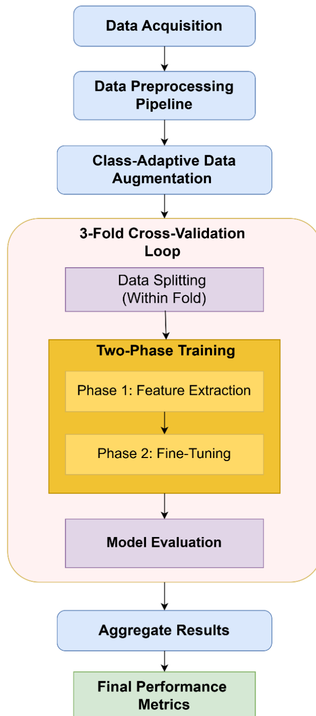
Fig. 1. Flowchart of Proposed Methodology
