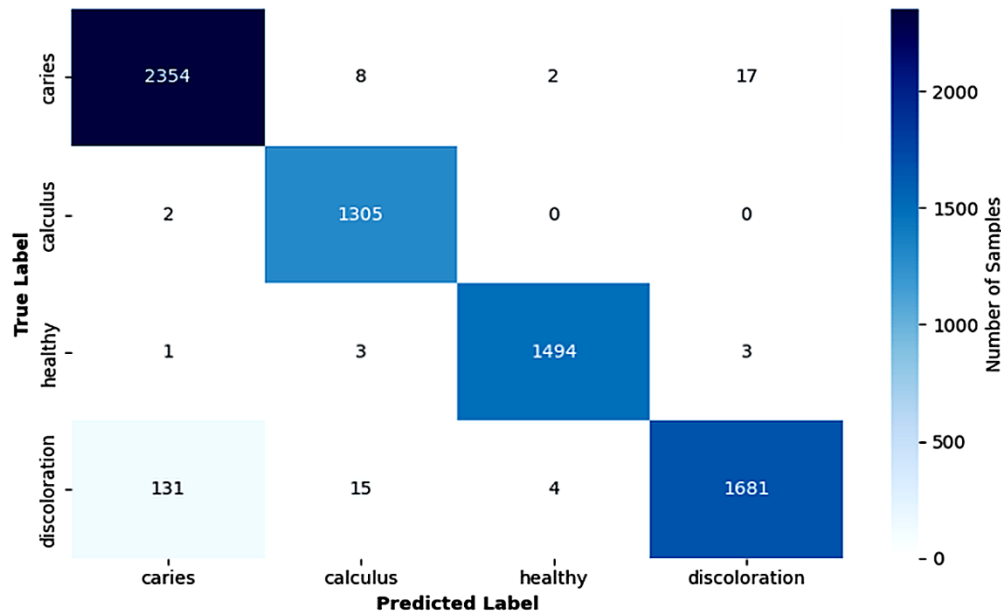
Fig. 4. Confusion Matrix
