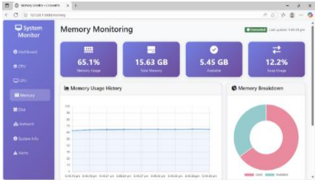
Figure 3. Memory and Disk Utilization Dashboard.
