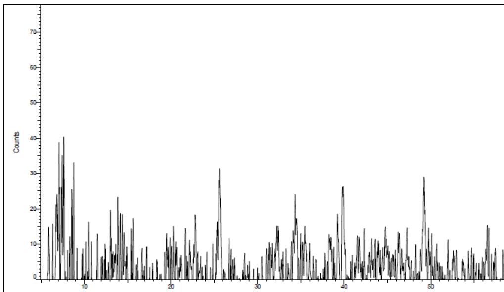
Figure 1. XRD of Coal Fly Ash (CFA)
