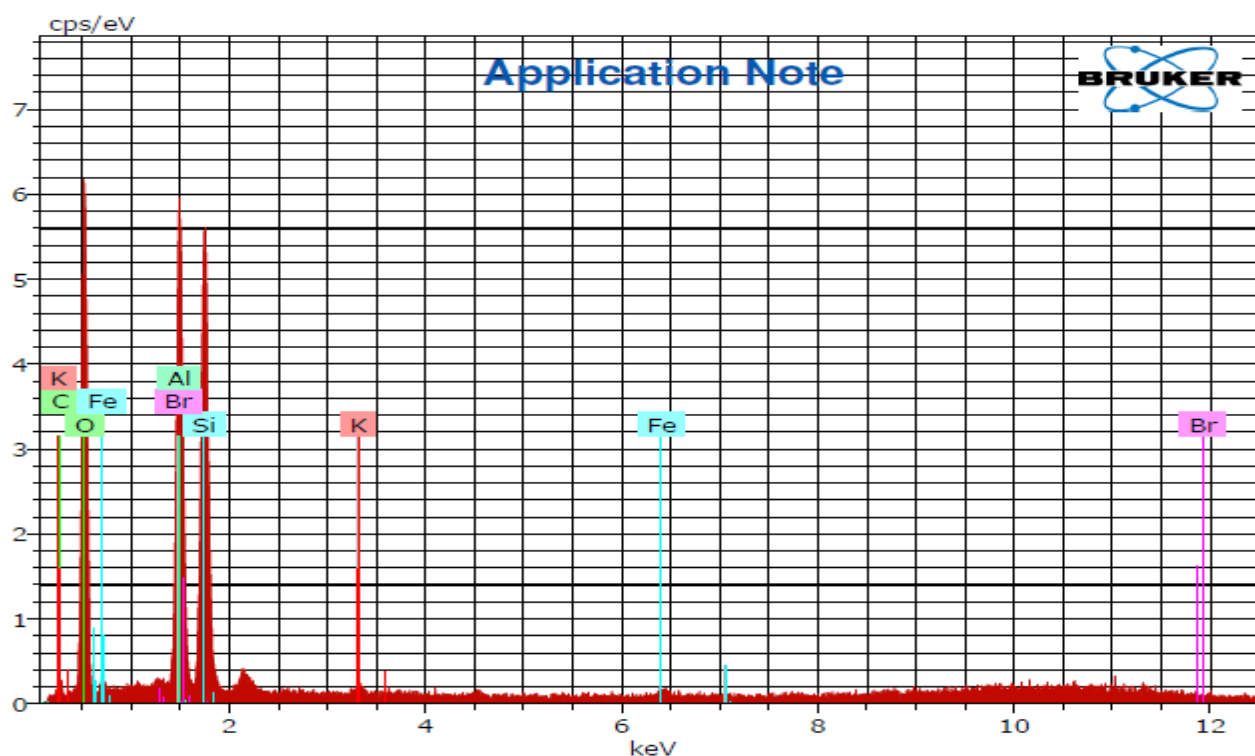
Fig.8 EDAX of fly ash
