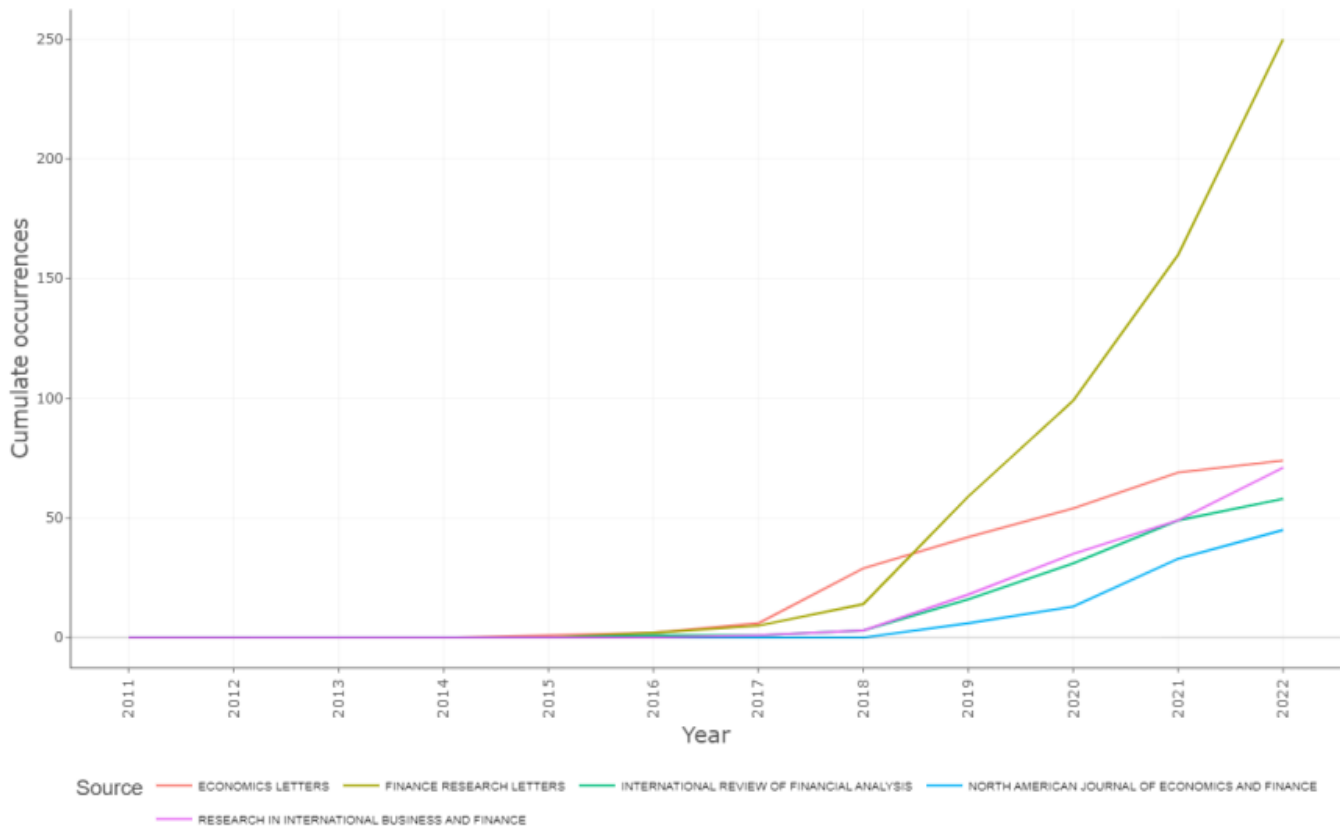
Figure 5 – Source Dynamics
