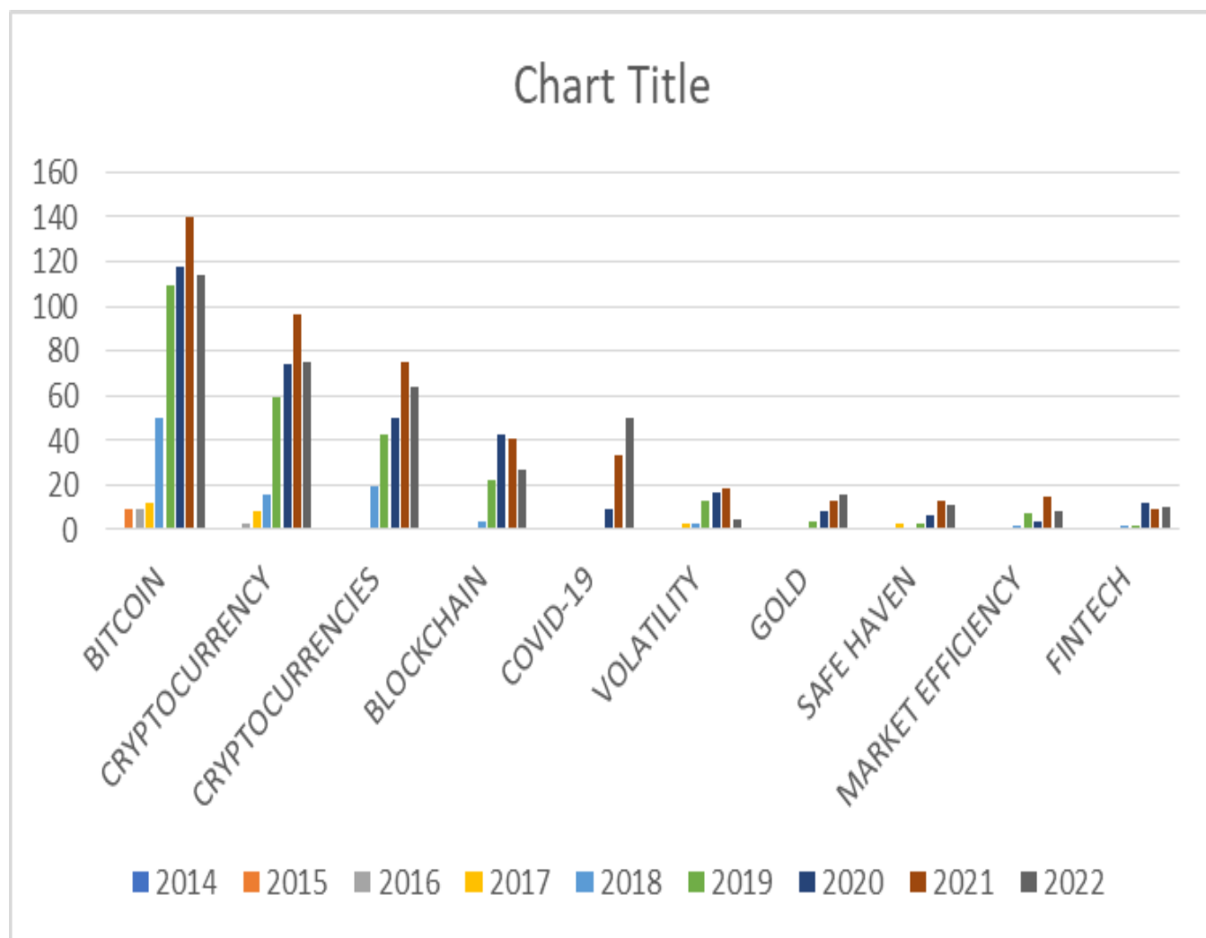
Figure 9- Word Dynamics
