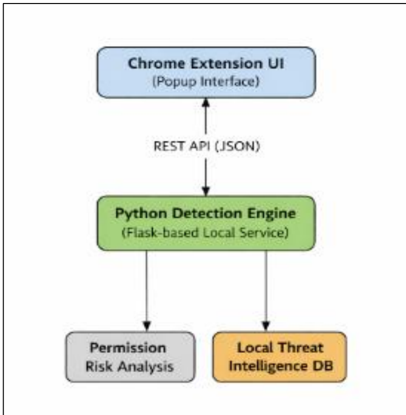
Fig1: Single column system architecture of the Proposed hybrid static analysis framework
