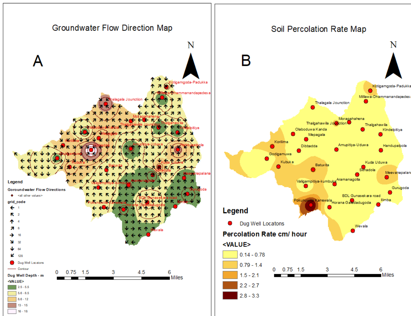
Figure 06 A – Groundwater Flow Direction Map, B - Soil Percolation Rate (cm/hour) Map
