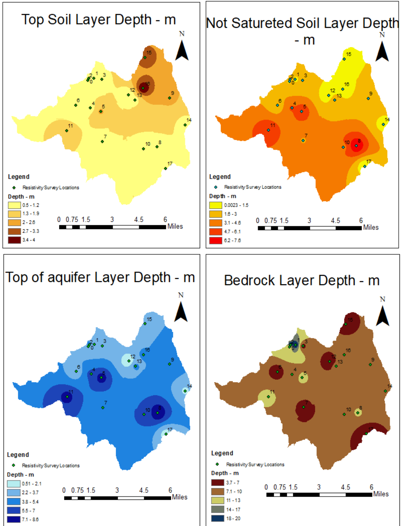
Figure 03 Electrical Sounding Resistivity Layer Maps
