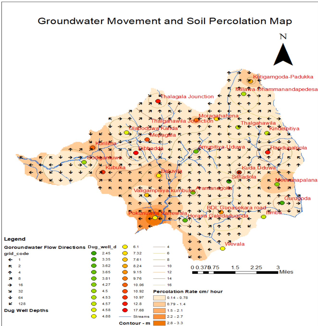
Figure 07 Groundwater Movement and Soil Percolation
