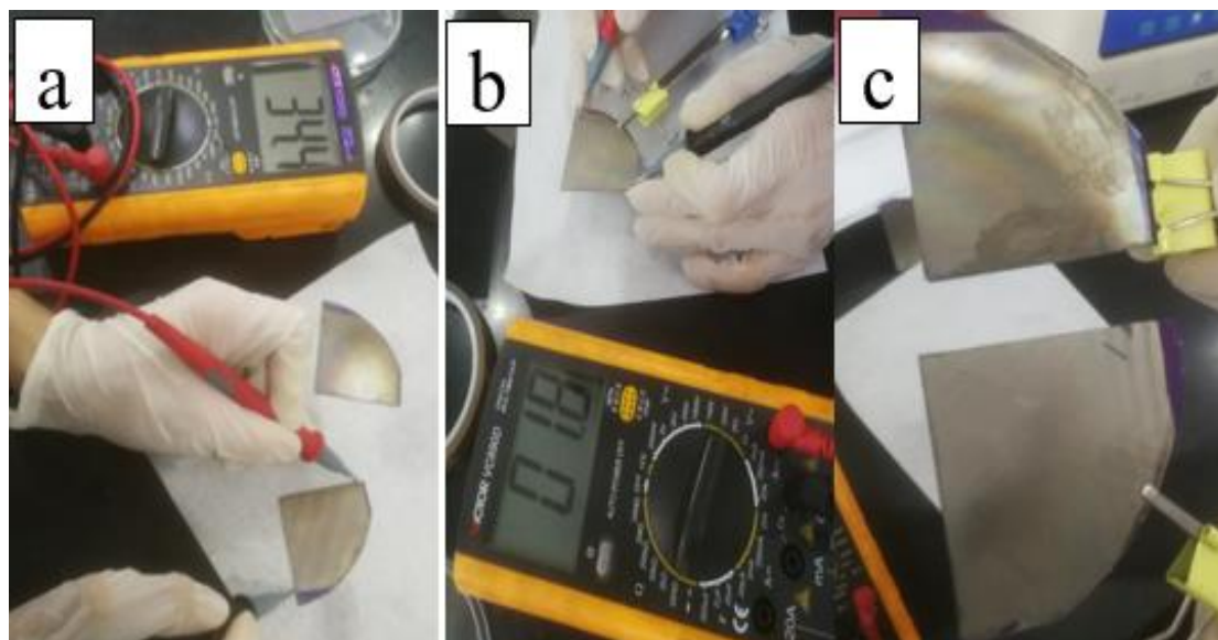
Figure 3. 2(a) Resistance before nickel deposition, figure 3.2(b) Resistance after nickel deposition, and figure 3.2(c) Comparison between the surface of the substrate electrode with and without nickel deposited .
