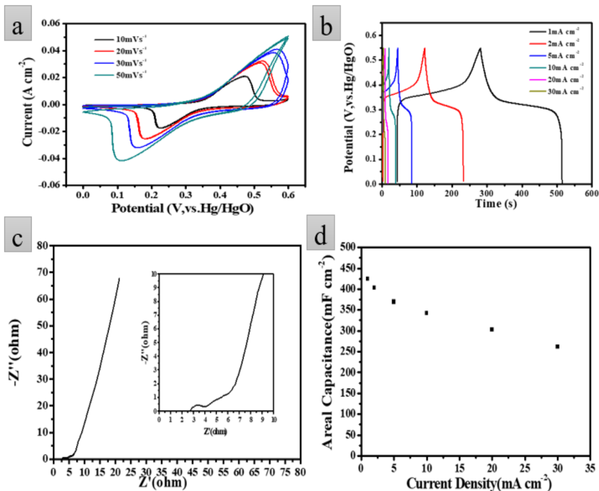
Figure 3. 4 (a) CV curves at various scan rates inside 2M KOH electrolyte, figure 3.4(b) Charge-discharge curves for NiCo-LDH in 2M KOH electrolyte at different current densities, figure 3.4(c) electrochemical impedance spectroscopy in 2M KOH electrolyte and figure 3.4(c) Areal capacitance of NiCo-LDH in 2M KOH electrolyte at different current densities.
