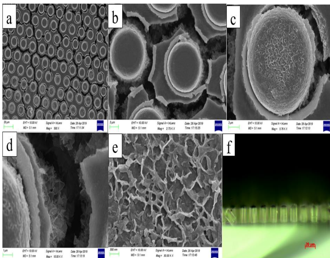
Figure 3. 3: Scanning Electron Microscopy images of NiCo-LDH.
