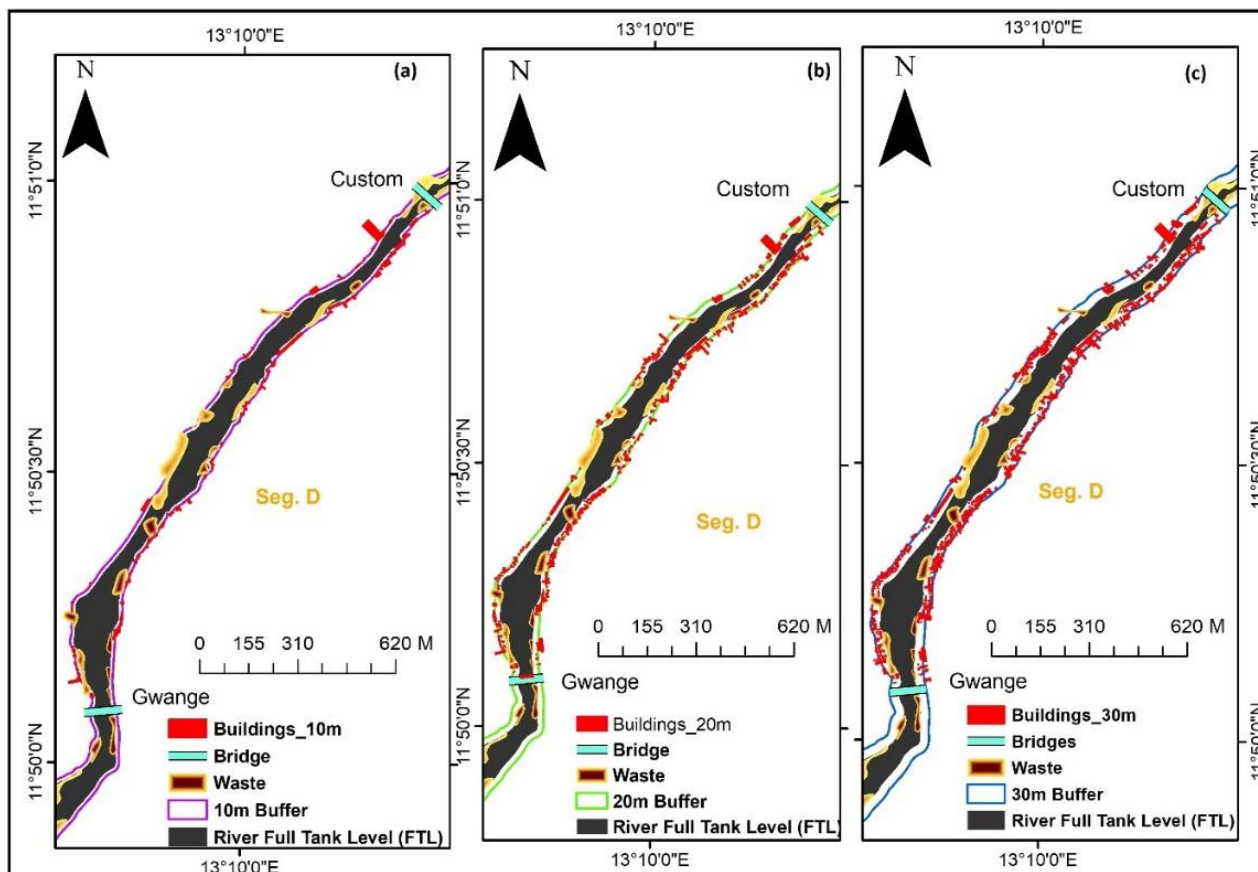
Figure 8. Buildings encroachment within (a) 10 m, (b) 20 m, and (c) 30 m river buffer zones along Segment D
