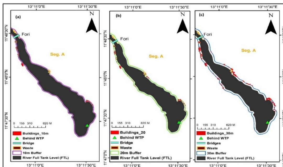
Figure 5. Buildings encroachment within (a) 10 m, (b) 20 m, and (c) 30 m river buffer zones along Segment A
