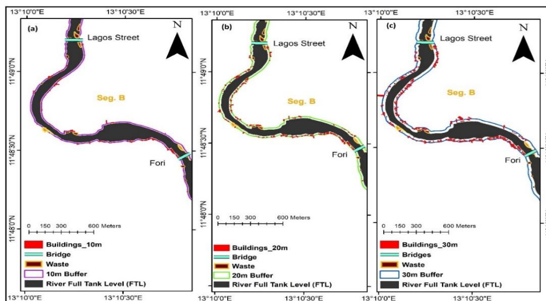
Figure 6. Buildings encroachment within (a) 10 m, (b) 20 m, and (c) 30 m river buffer zones along Segment B
