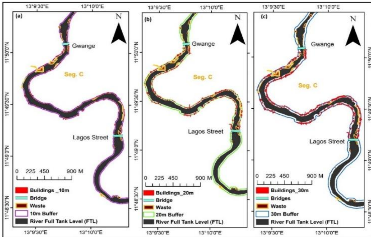
Figure 7. Buildings encroachment within (a) 10 m, (b) 20 m, and (c) 30 m river buffer zones along Segment C
