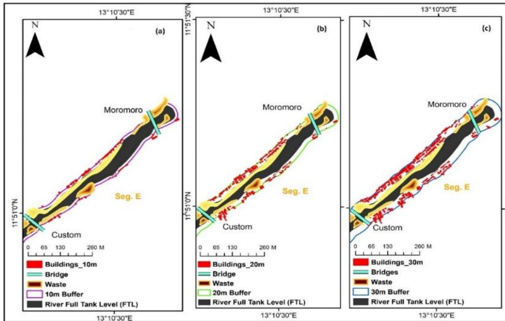
Figure 9. Buildings encroachment within (a) 10 m, (b) 20 m, and (c) 30 m river buffer zones along Segment E
