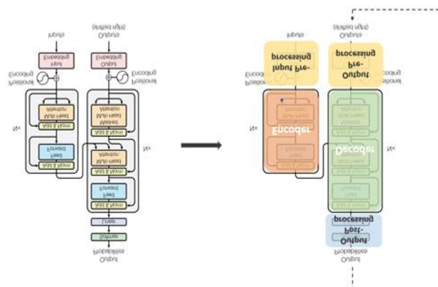
Figure. 3. Transformer Architecture
