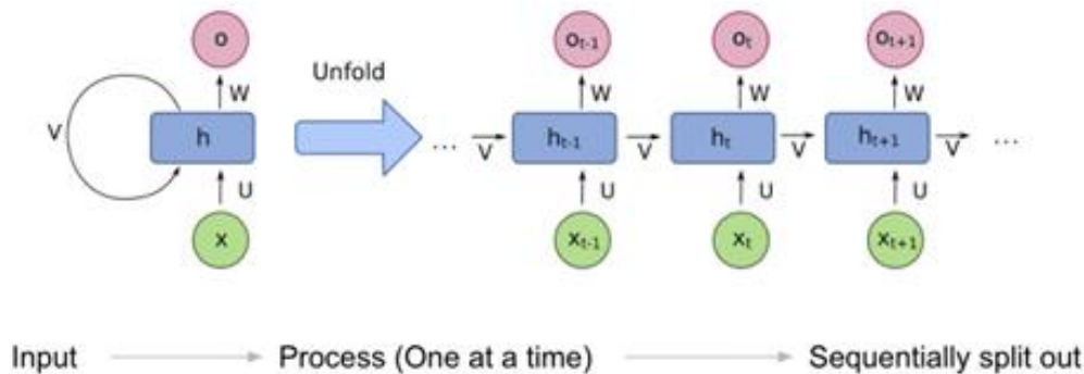
Figure 2. RNN- Handling sequence data.
