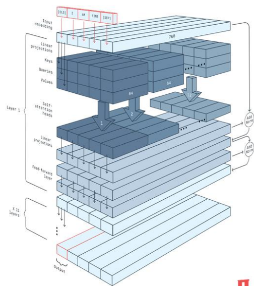
Figure 4. BERT Encoding.
