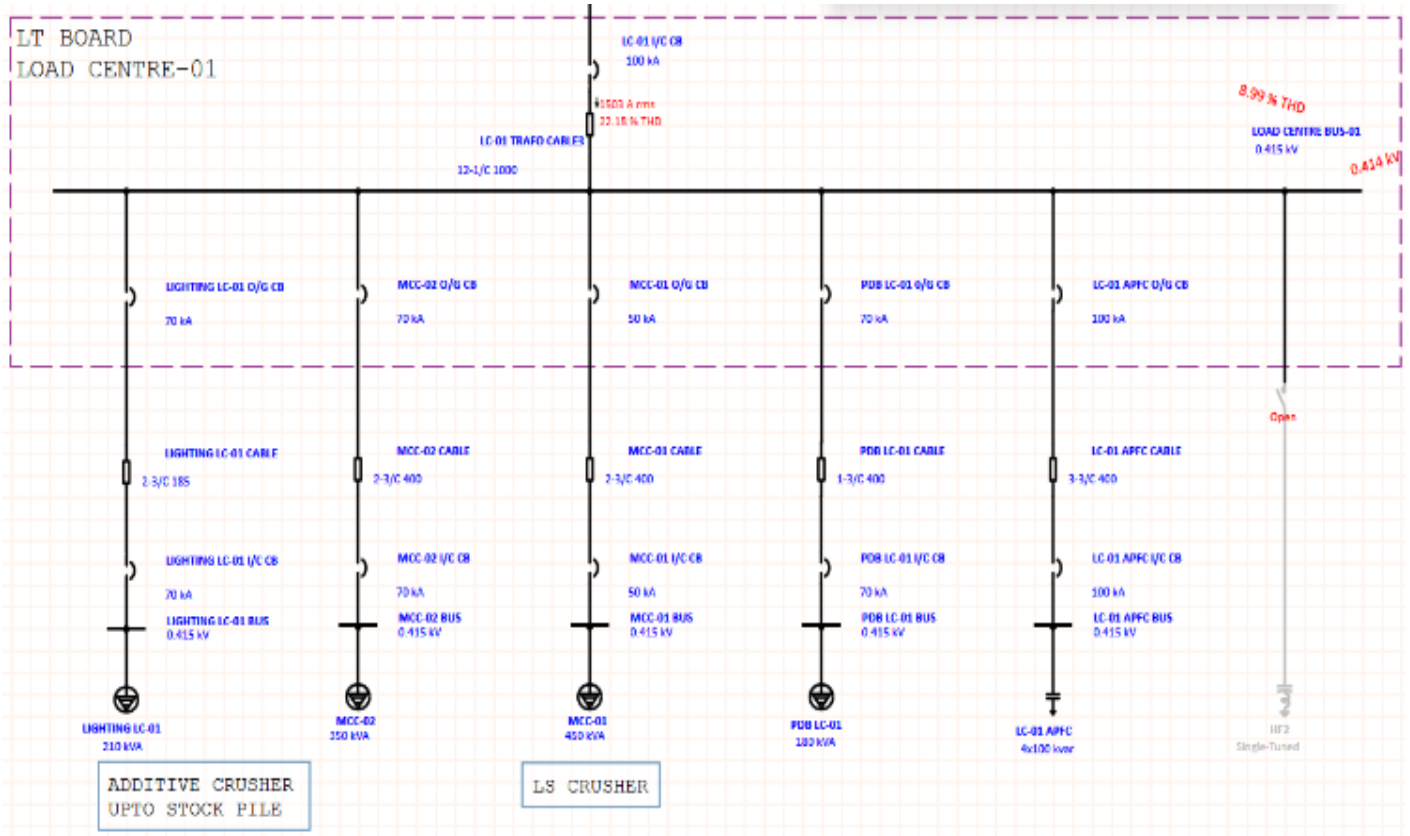
Figure 3: THD level at Load Centre-01 bus before mitigation
