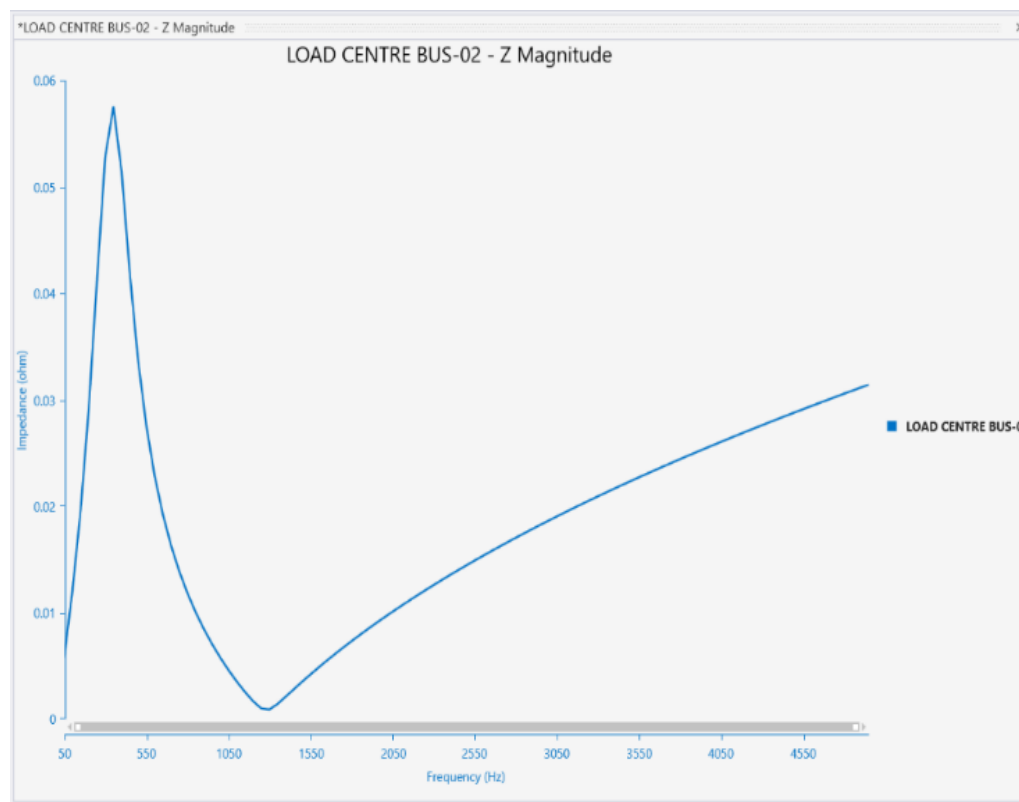
Figure 5: Parallel Resonance condition
