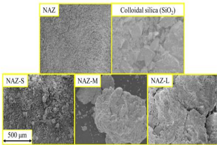
Figure 2. SEM images of prepared absorbents [27]
