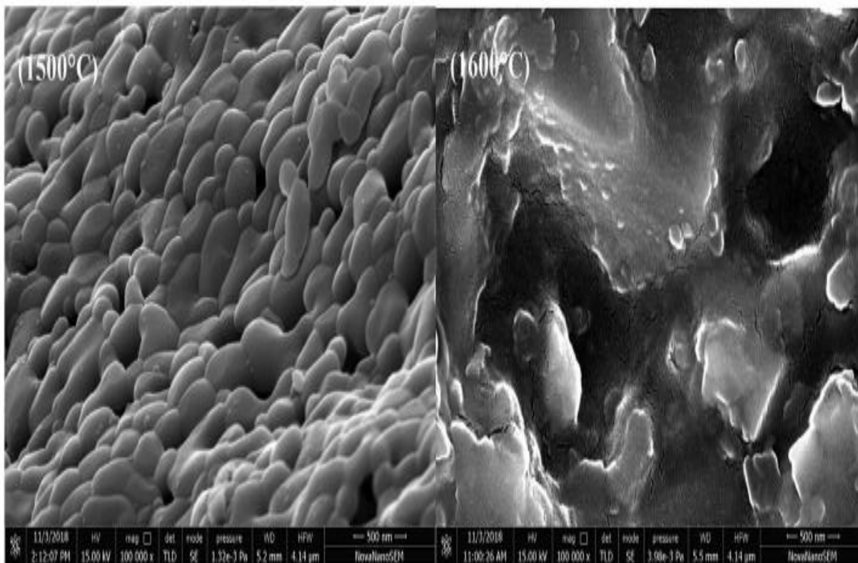
Figure 4. SEM micrograph of sintered lakargiite surfaces at 1500°C and 1600°C [43]
