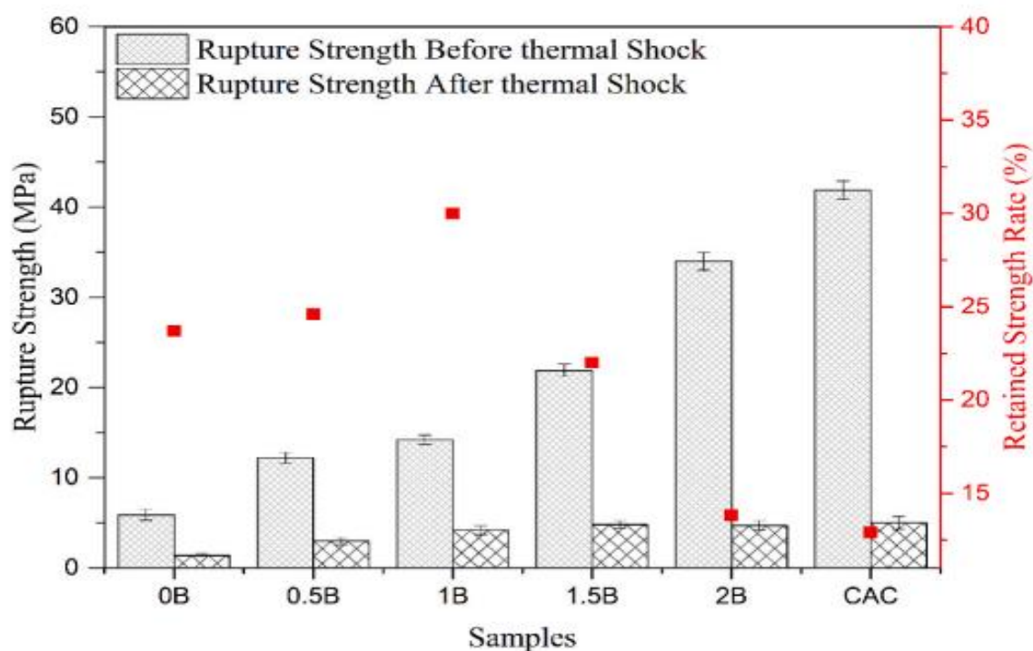
Figure 3. The castables' residual strength rate [37]
