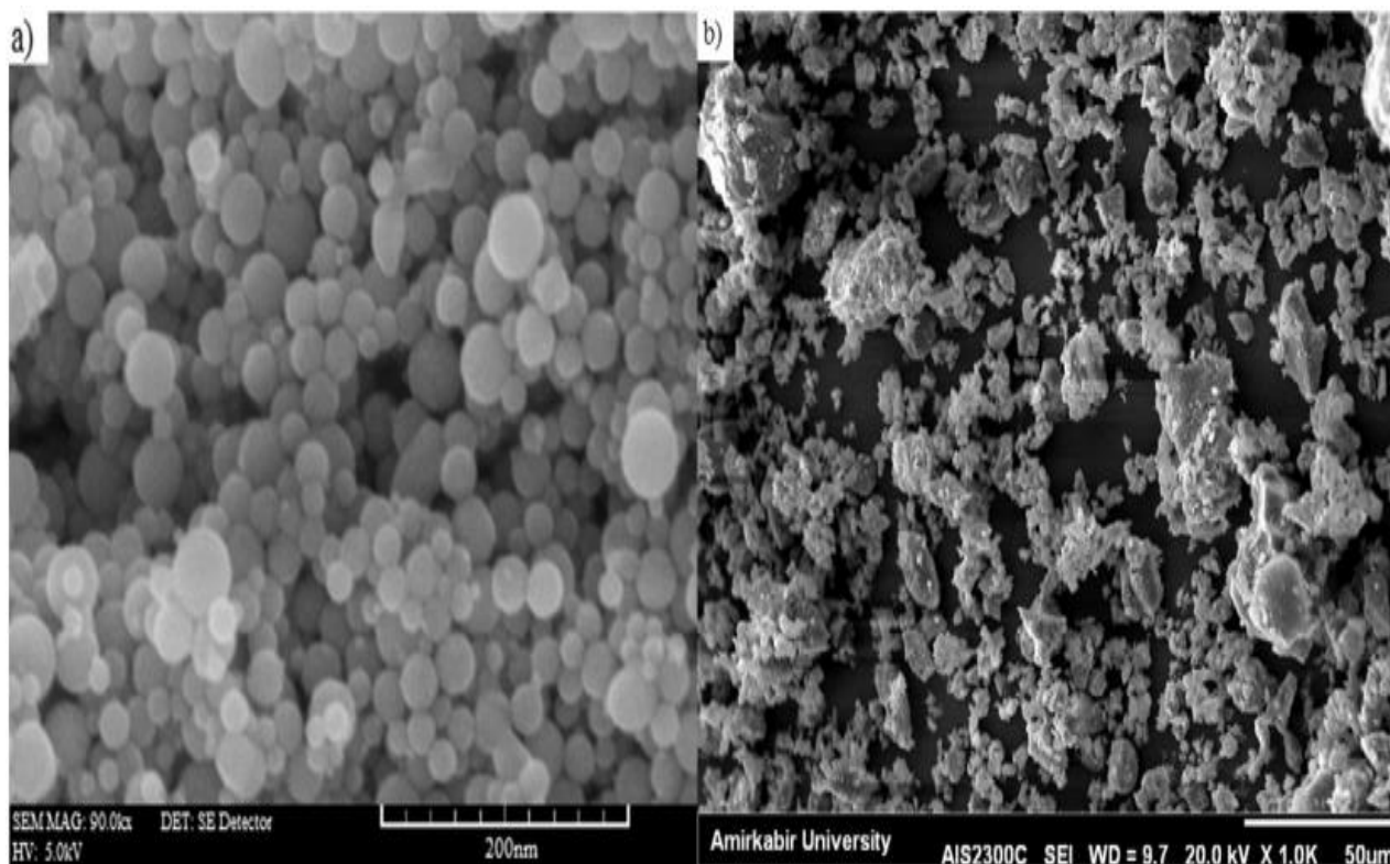
Figure 1. (a) SEM images of NA (b) SEM images of RHA particles [24]
