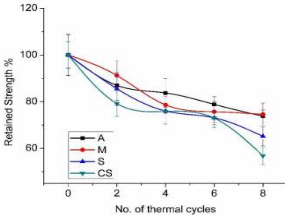
Figure 5. Silica sol bound castables are resistant to thermal shock in batches that have been produced and contain sol [48]
