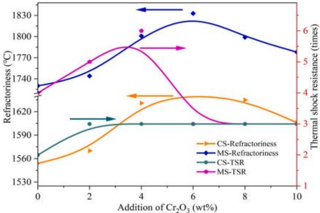
Figure 7.impact of \text{Cr}_2\text{O}_3 addition on thermal shock resistance and refractoriness of refractory materials made using microwave and traditional sintering techniques [62]
