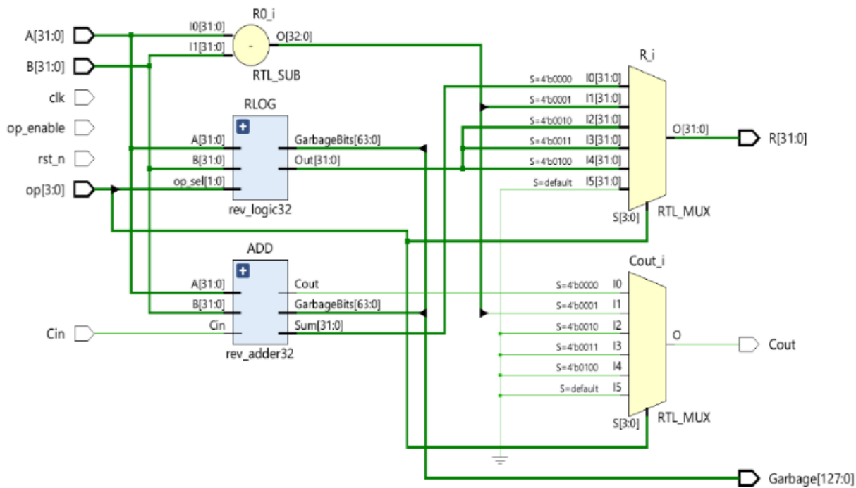
Figure 8: Reversible RTL Schematic
