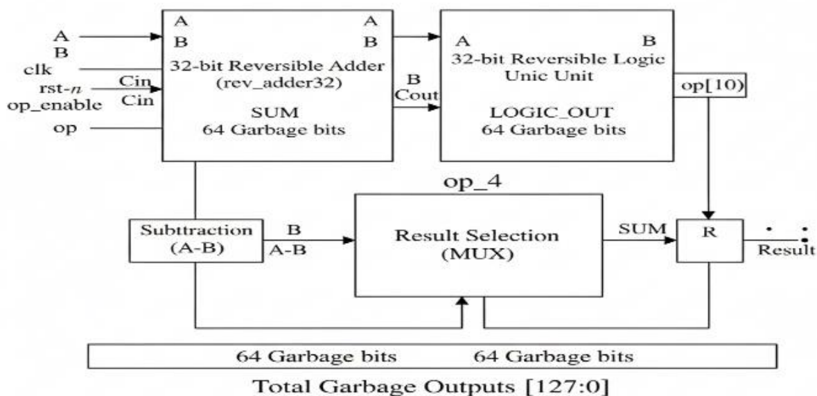
Figure 7: Reversible 32-bit
