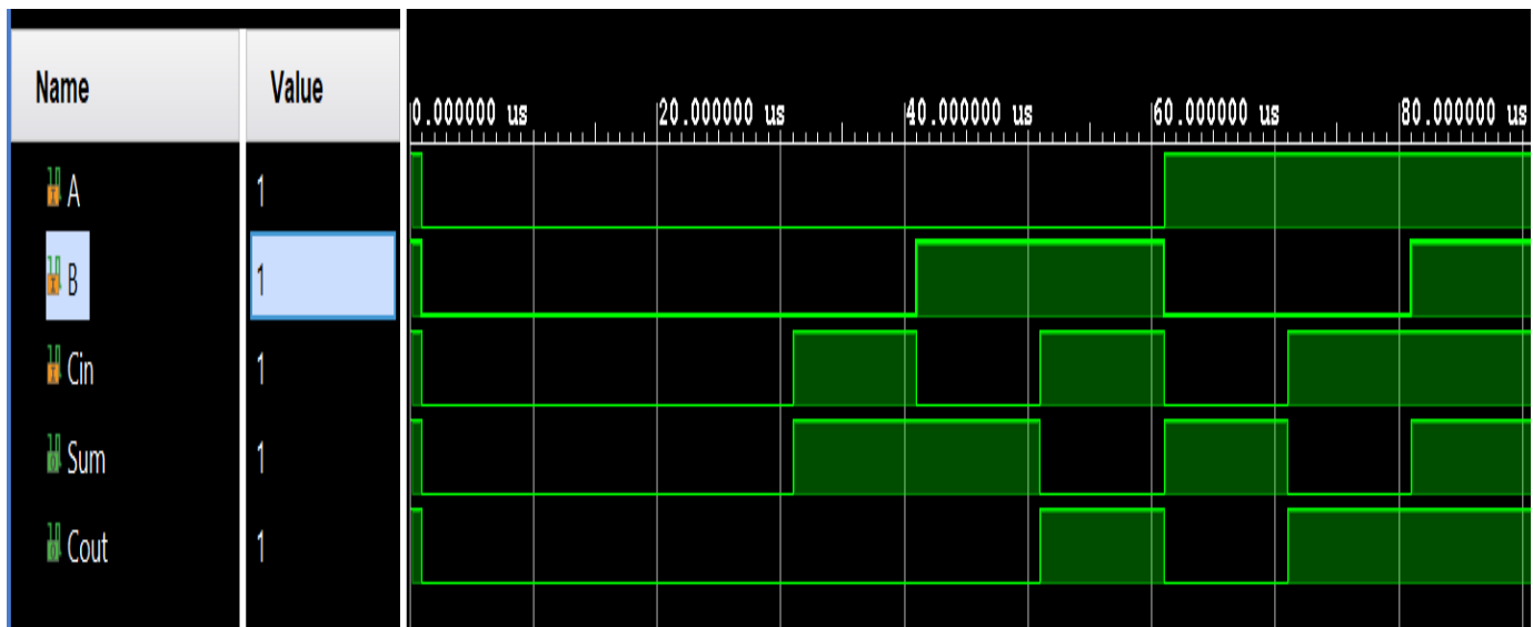
Figure 11: 32-bit output of Full Adder
