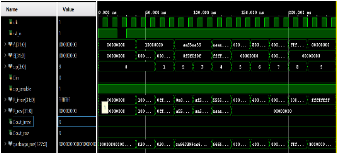
Figure 10: 32-bit output of Full Adder Using reversible gates
