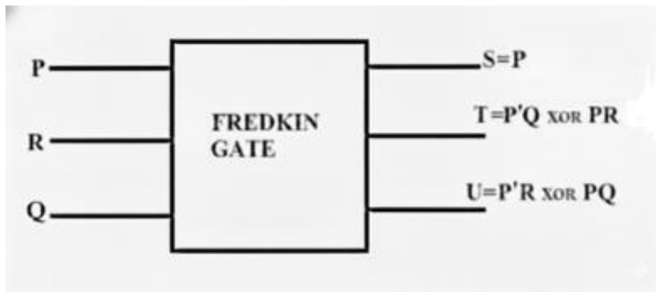
Figure 5: Fredkin Gate
