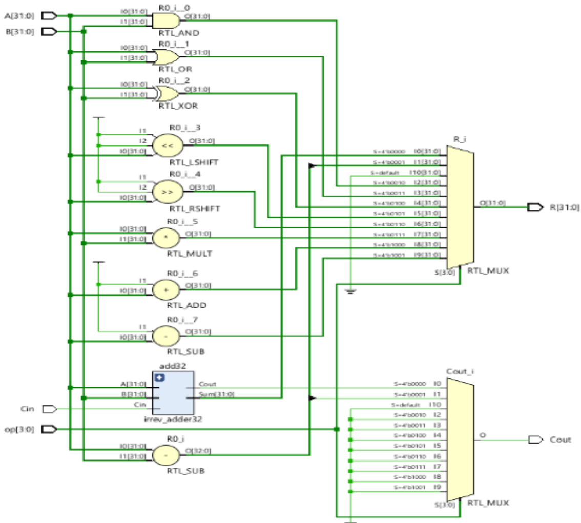
Figure 9: Irreversible RTL Schematic
