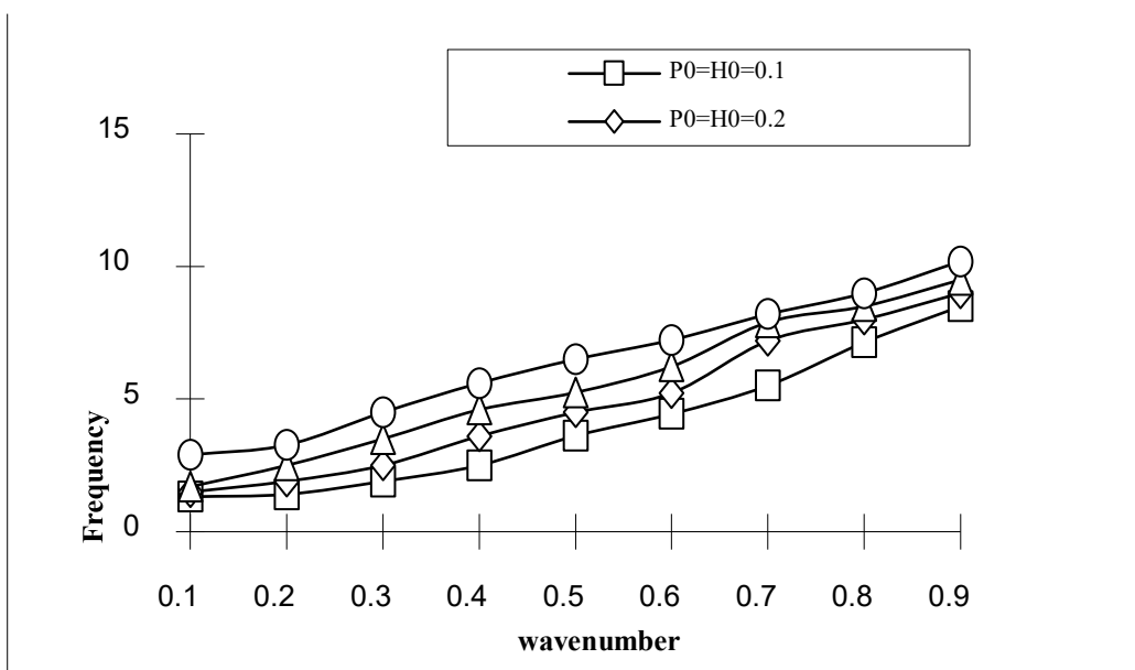
Fig:4 Variation of frequency with wavenumber for Material-I at ( \theta = 60^\circ )
