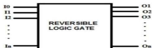
Fig. 3.1. Reversible Logic
