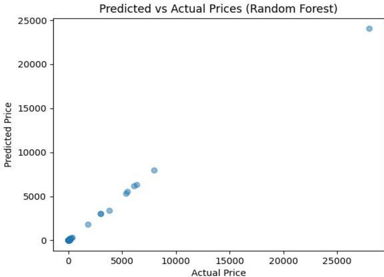
Predicted vs Actual Prices (Random Forest)
