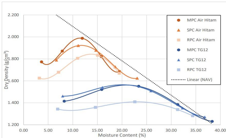
Figure 9. Dry Density ( \text{g/cm}^3 ) vs Moisture Content for all compaction test
