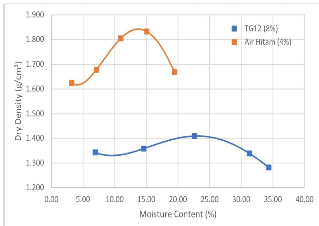
Figure 7. Dry Density ( \text{g/cm}^3 ) vs Moisture Content for RPC
