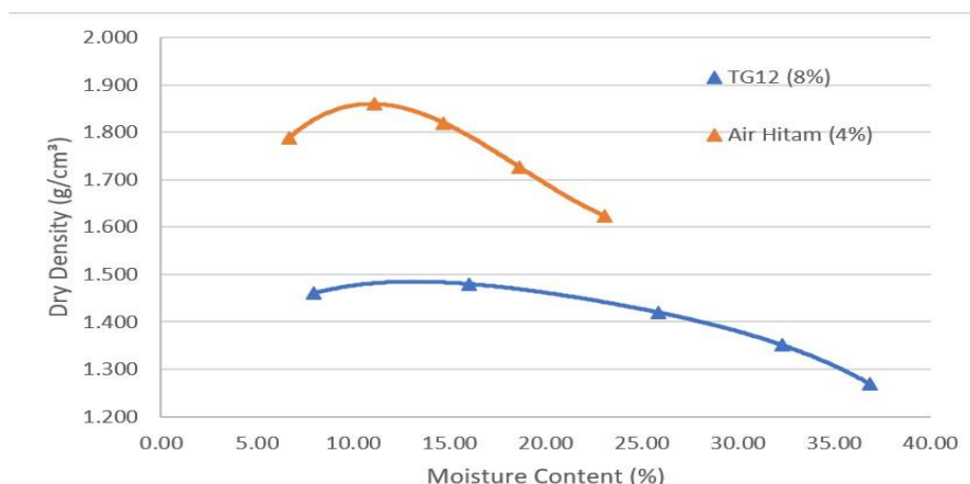
Figure 6. Dry Density (g/cm 3 ) vs Moisture Content for SPC
