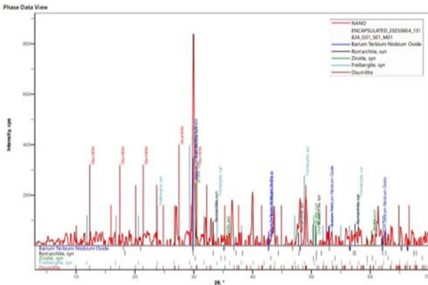
Figure 8 X –ray Diffraction spectral
