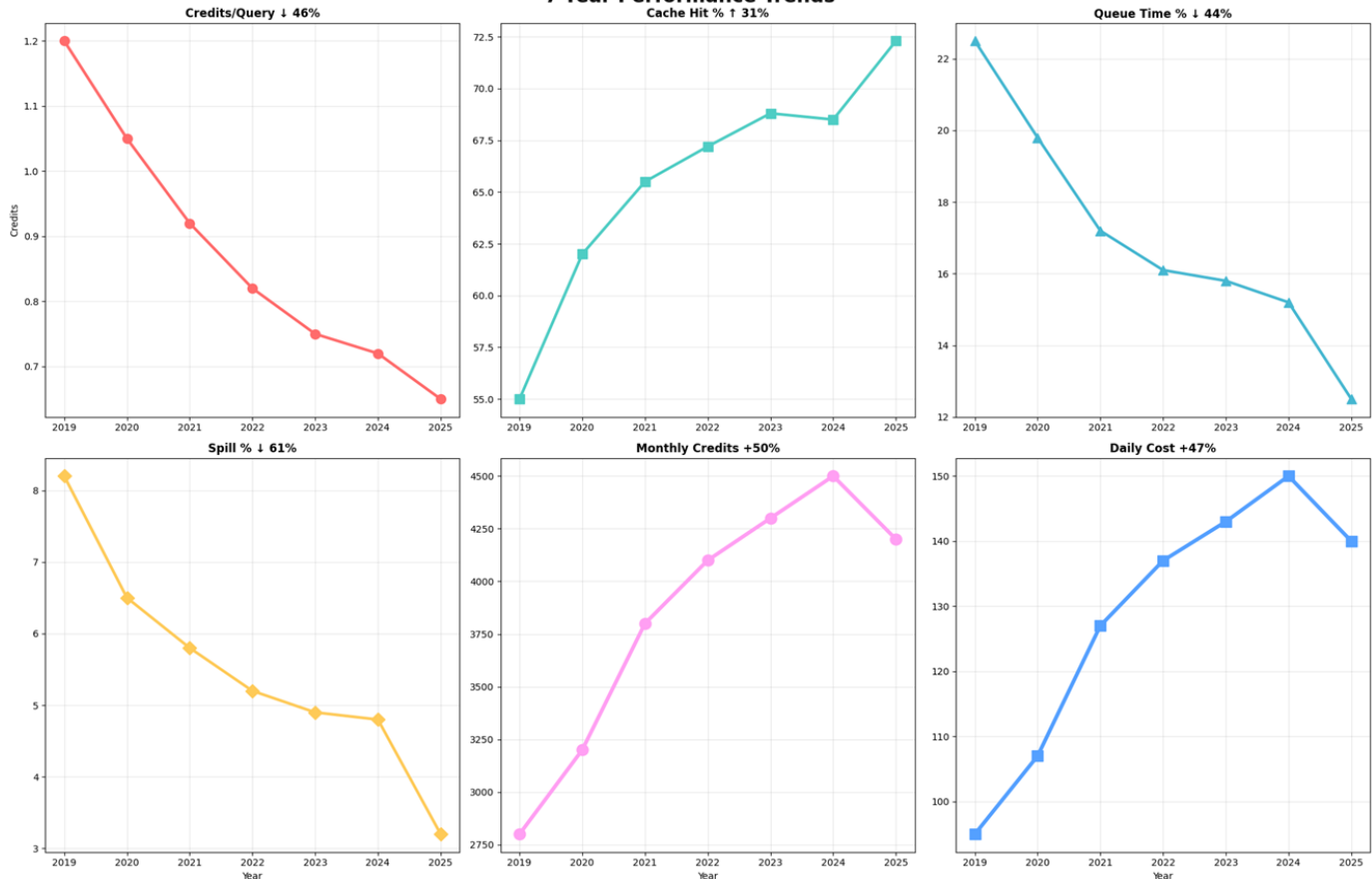
Figure 2: Snowflake Cost Evaluation
