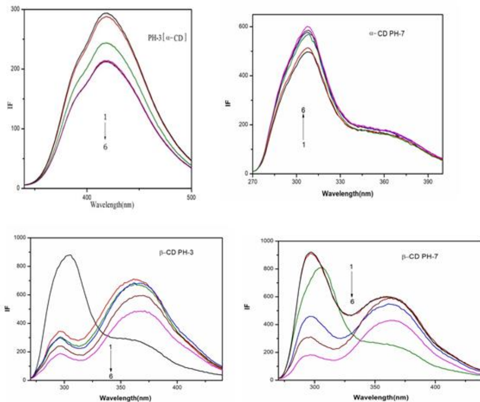
Fig. 2 Fluorescence spectra of 2PDA in different \alpha -CD and \beta -CD concentrations (M): 0, (2) 0.002, (3) 0.004, (4) 0.006, (5) 0.008, (6) 0.01.
