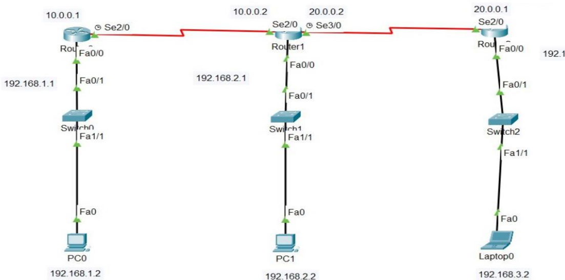
Figure 1. Dynamic Routing implementation using (OSPF)on Cisco Packet Tracert configured interface 1 (Router0) with Host 1 which is PC0 and the Serial port.
