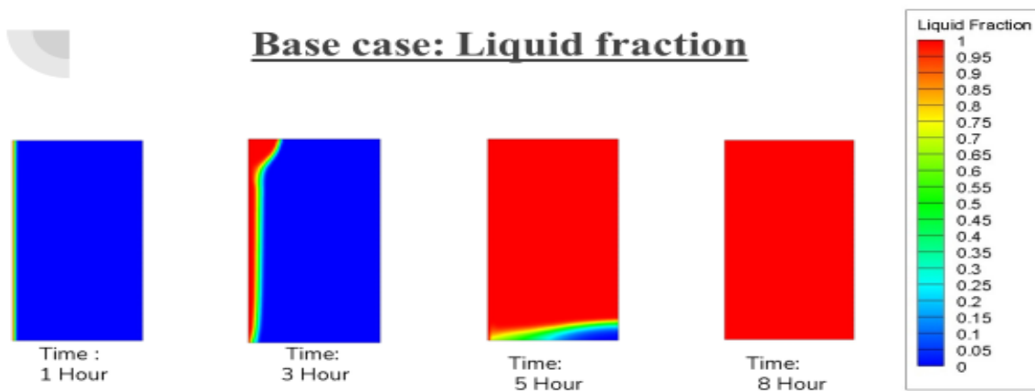
Figure:9 base case temperature curve for battery PCM liquid fraction with respect to discharge time
