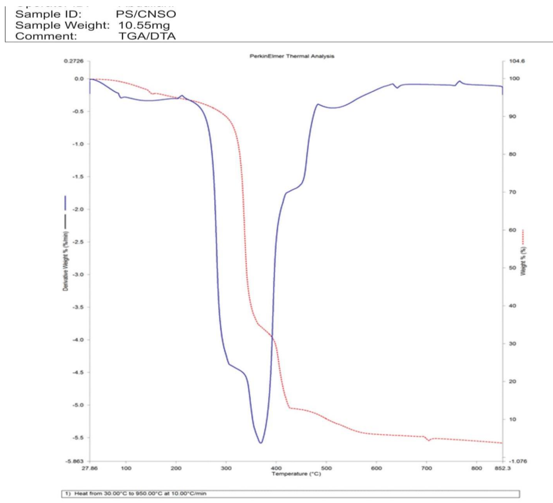
Figure 1 DTA analysis of PS/CNSO
