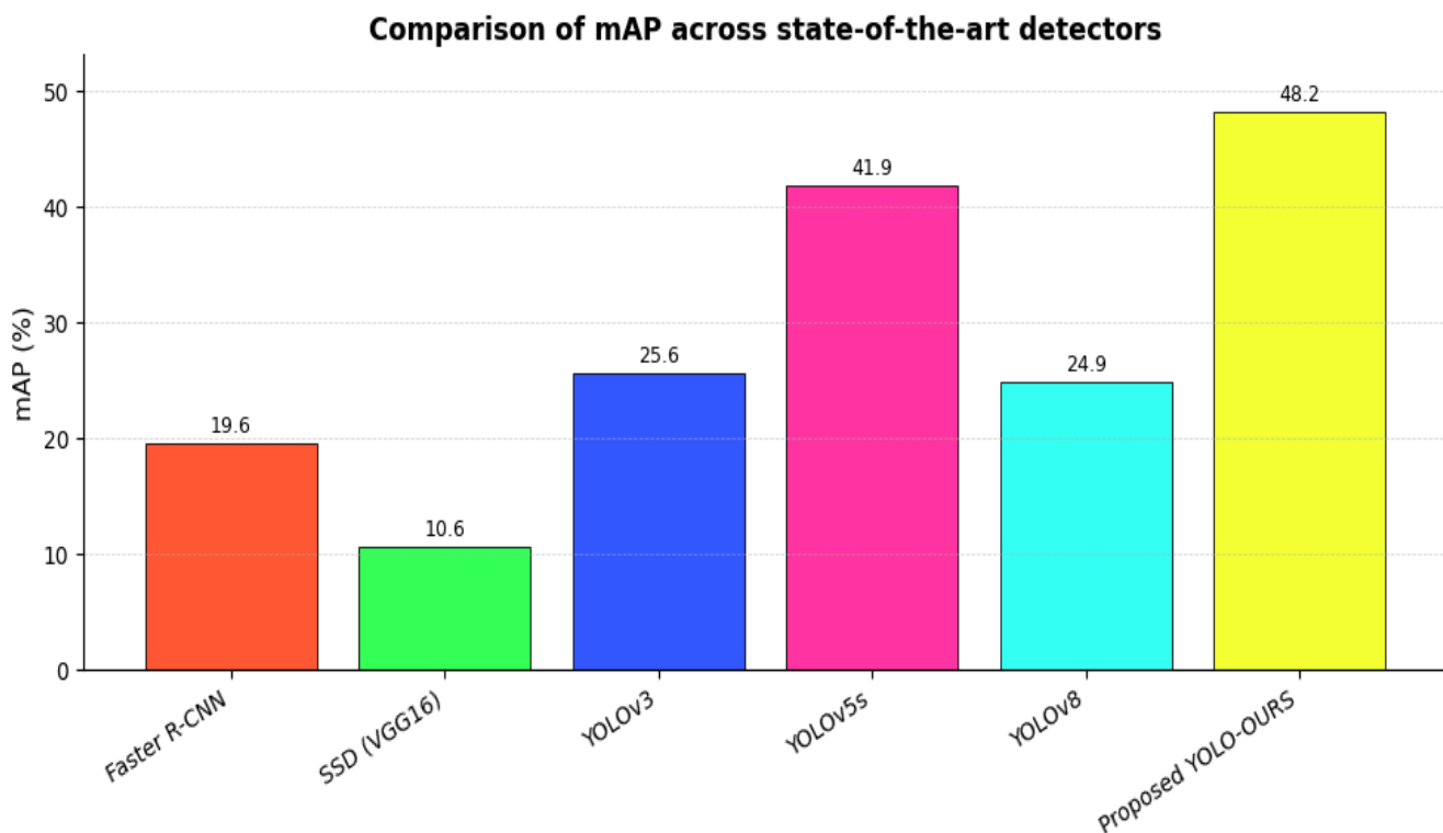
Figure 10: Comparison of mAP across state-of-the-art detectors.
