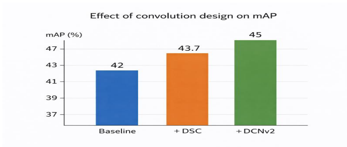
Figure 8: Effect of convolution design on mAP”, showing baseline, +DSC, and +DCNv2.
