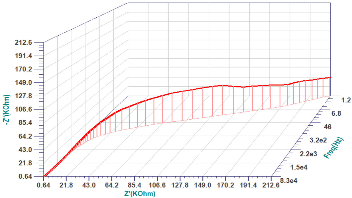
Figure 6: AC impedance spectra of 21K gold alloy immersed in artificial saliva.
