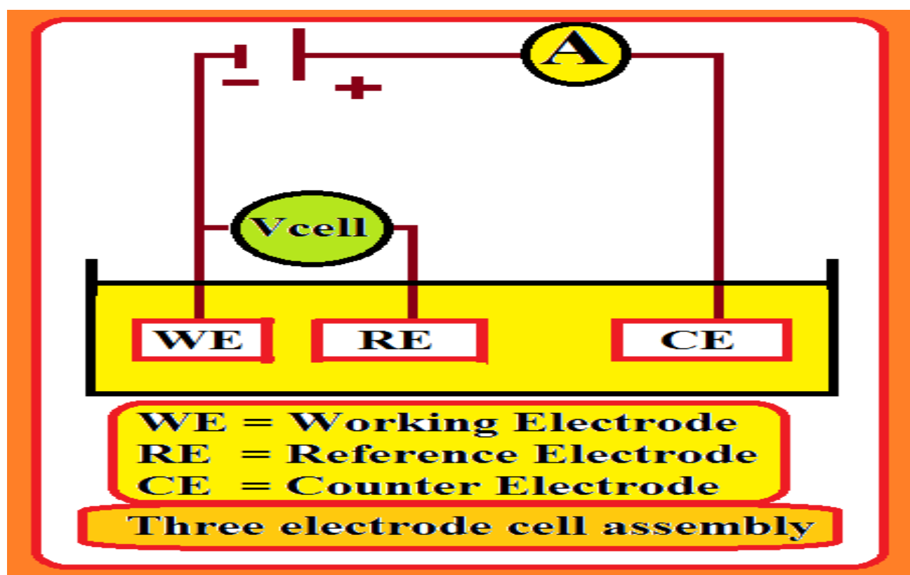
Figure 2. Three-electrode cell assembly
