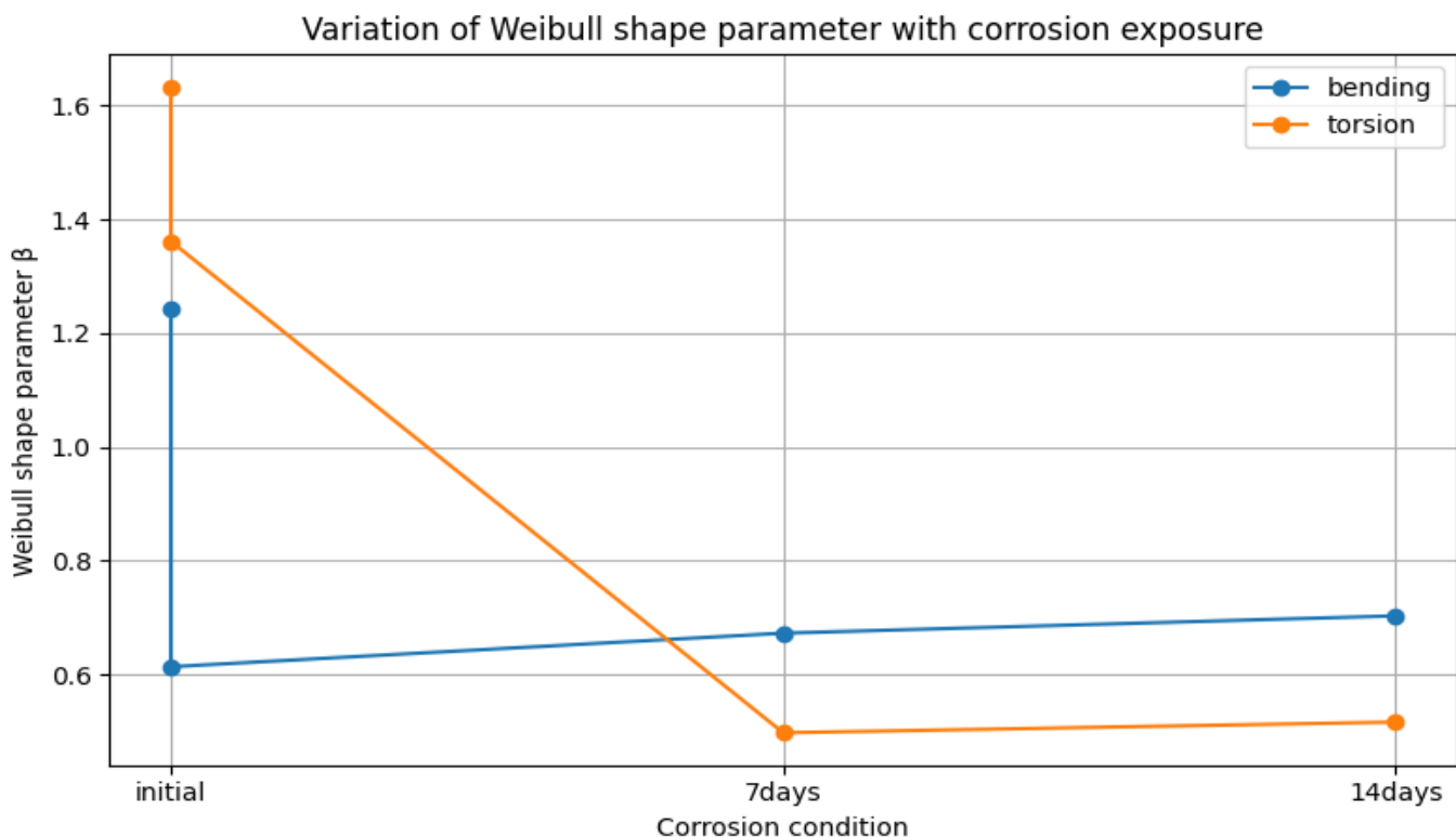
Figure 1: Variation of the Weibull shape parameter \beta with corrosion exposure for bending and torsional loading of AA 7075-T651.
