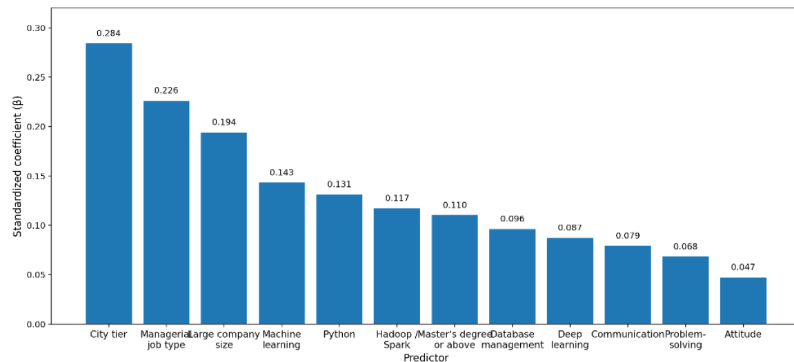
Figure 6. Standardized coefficients of non-zero predictors from the LASSO salary model.
