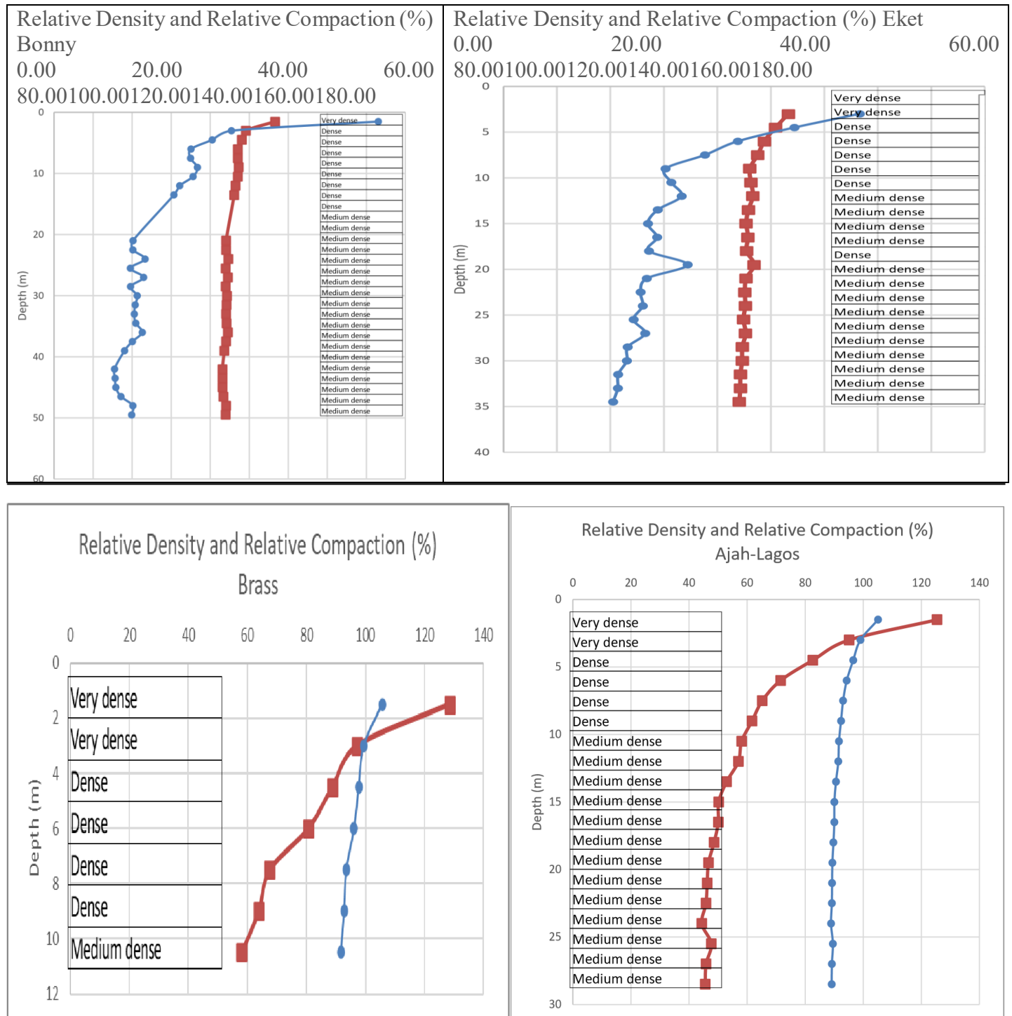
Fig.(14) Variation of Density related geotechnical parameters across the Nigerian Beach Ridge
