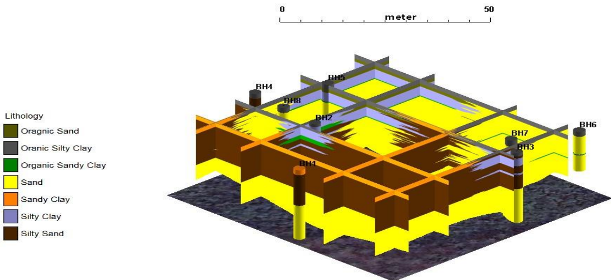
Fig.7: Composite Stratigraphy
