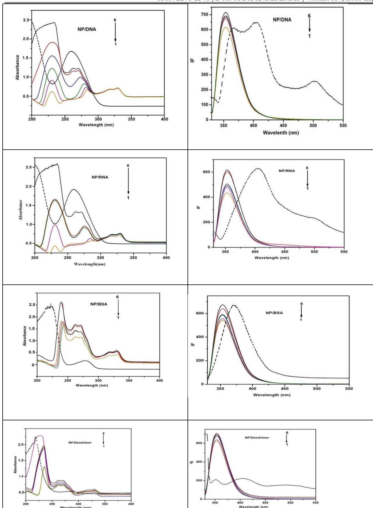
Fig.2. Absorption and fluorescence spectra of naproxen [0.2 x 10 -4 M] with different concentrations of biomolecules (DNA, RNA, BSA, Dendrimer) (M x 10 -6 ): 1) 0, 2) 2, 3) 4, 4) 6, 5) 8, 6) 10, dotted line indicates pure biomolecules spectra.
