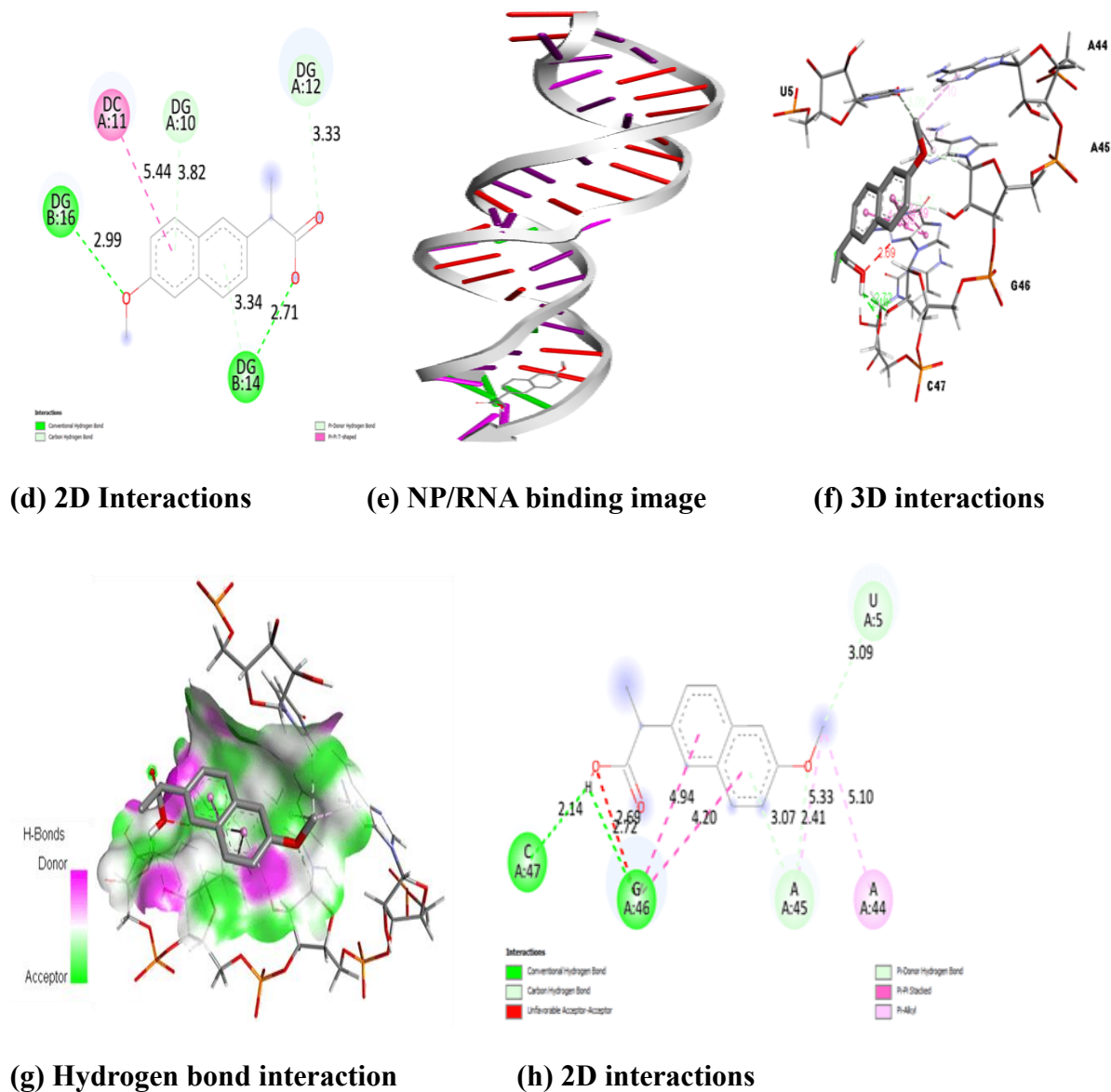
Fig. 3. Naproxen with biomolecule interaction images for (a-d) NP/DNA binding image, (e-h) NP/RNA binding images.
