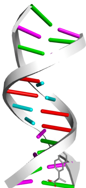
(a) NP/DNA binding image
