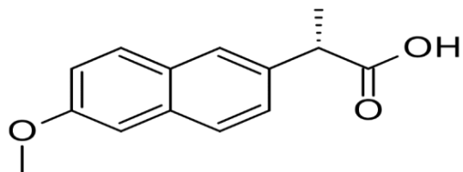
Fig. 1. Chemical structure of Naproxen
