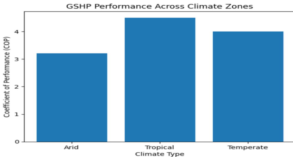
Graph 2 Climate Performance (COP vs climate)
