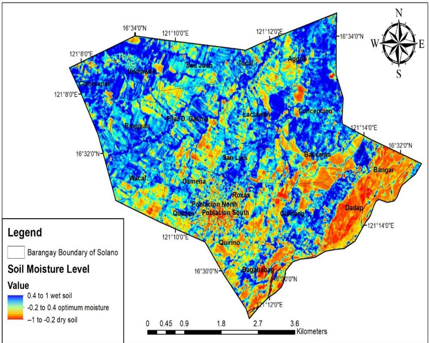
Figure 3. Soil Moisture Map of Solano, Nueva Vizcaya for the year 2020
