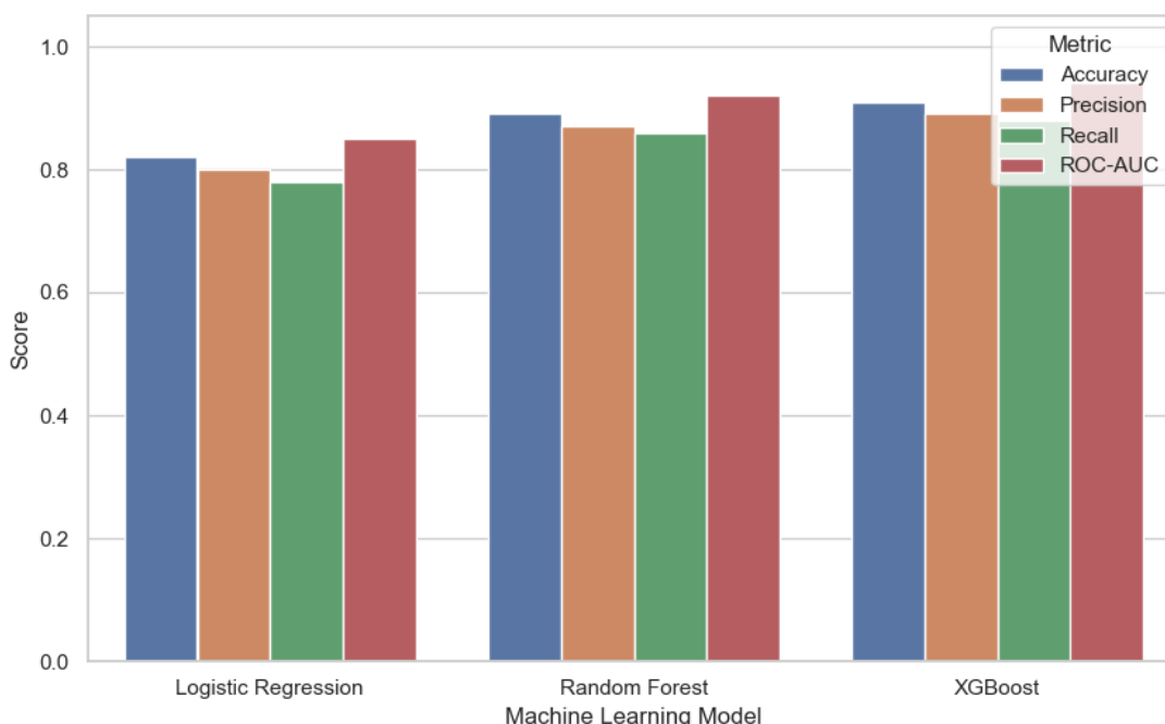
Figure 1: Performance comparison of ML Models for Early Asthma Detection
