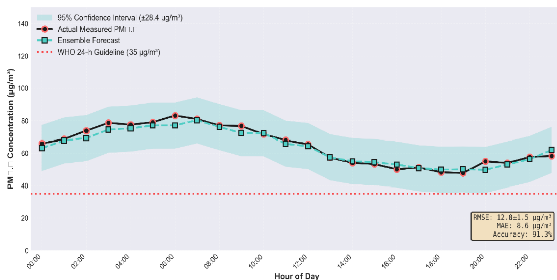
Fig. 4. Example 24-hour PM 2.5 forecast with ensemble model predictions (blue line) and 95% confidence intervals (shaded region). Observations from reference instruments are shown as red dots. The shaded uncertainty band (mean width: 28.4 µg/m³) reflects model prediction variance and is computed through Quantile Regression Forest post-processing. This case study demonstrates the model's ability to capture both rapid pollution onset during evening stagnation events and daytime ventilation patterns controlled by atmospheric mixing height dynamics.
