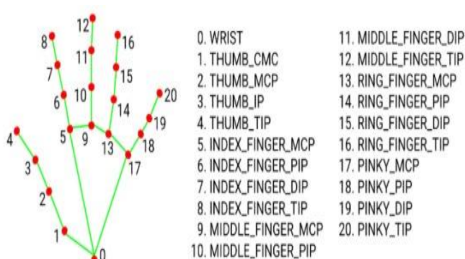
Fig 2: Hand Landmark Representation using MediaPipe
