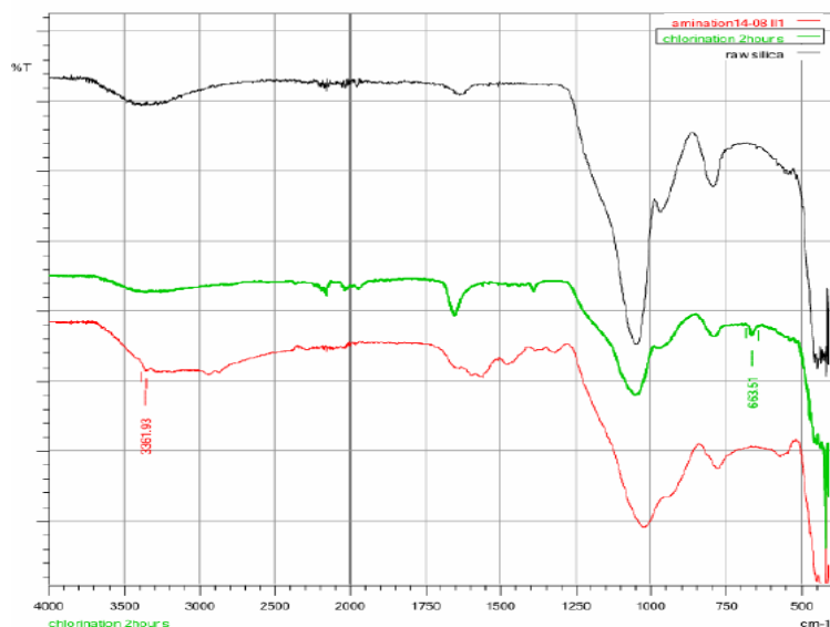
Figure 3.1: FT-IR spectra of raw silica, chlorinated, and aminated silica overlaid spectra
