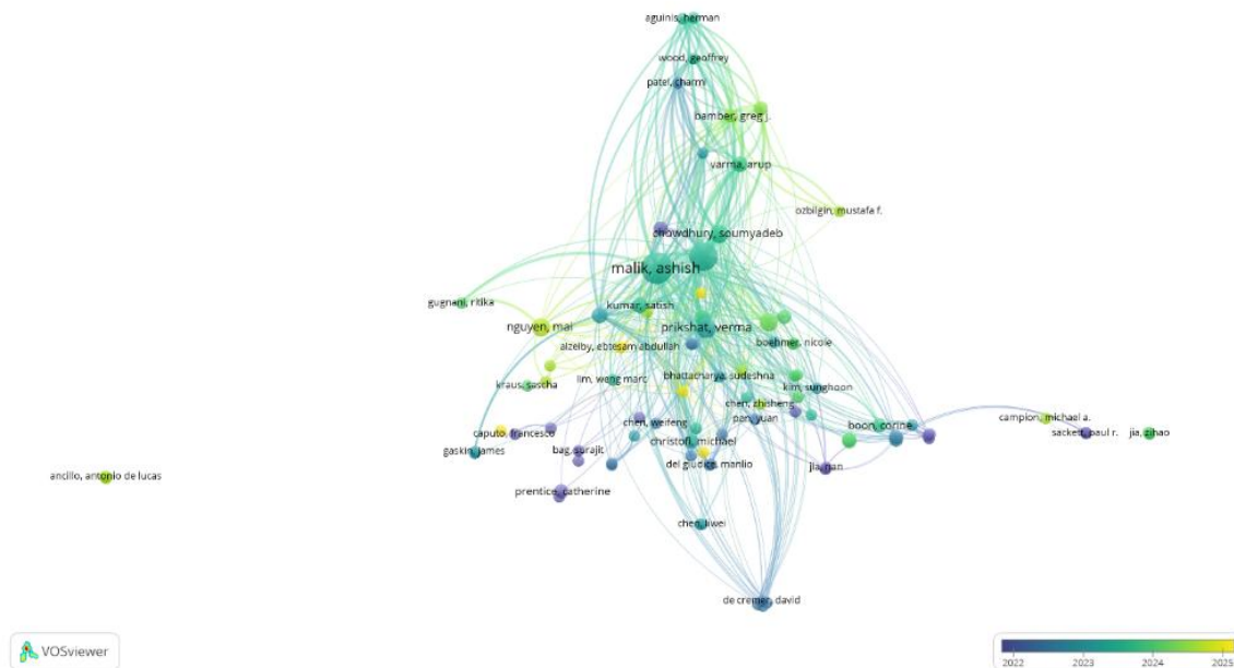
Figure 11: Bibliographic Coupling Analysis
