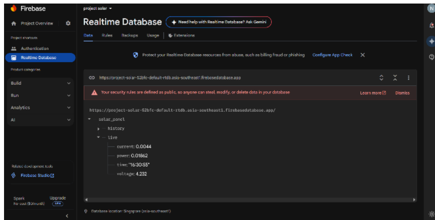
Figure 4. Firebase Interface
