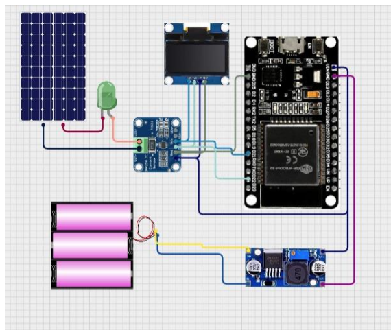
Figure 1. Circuit Diagram
