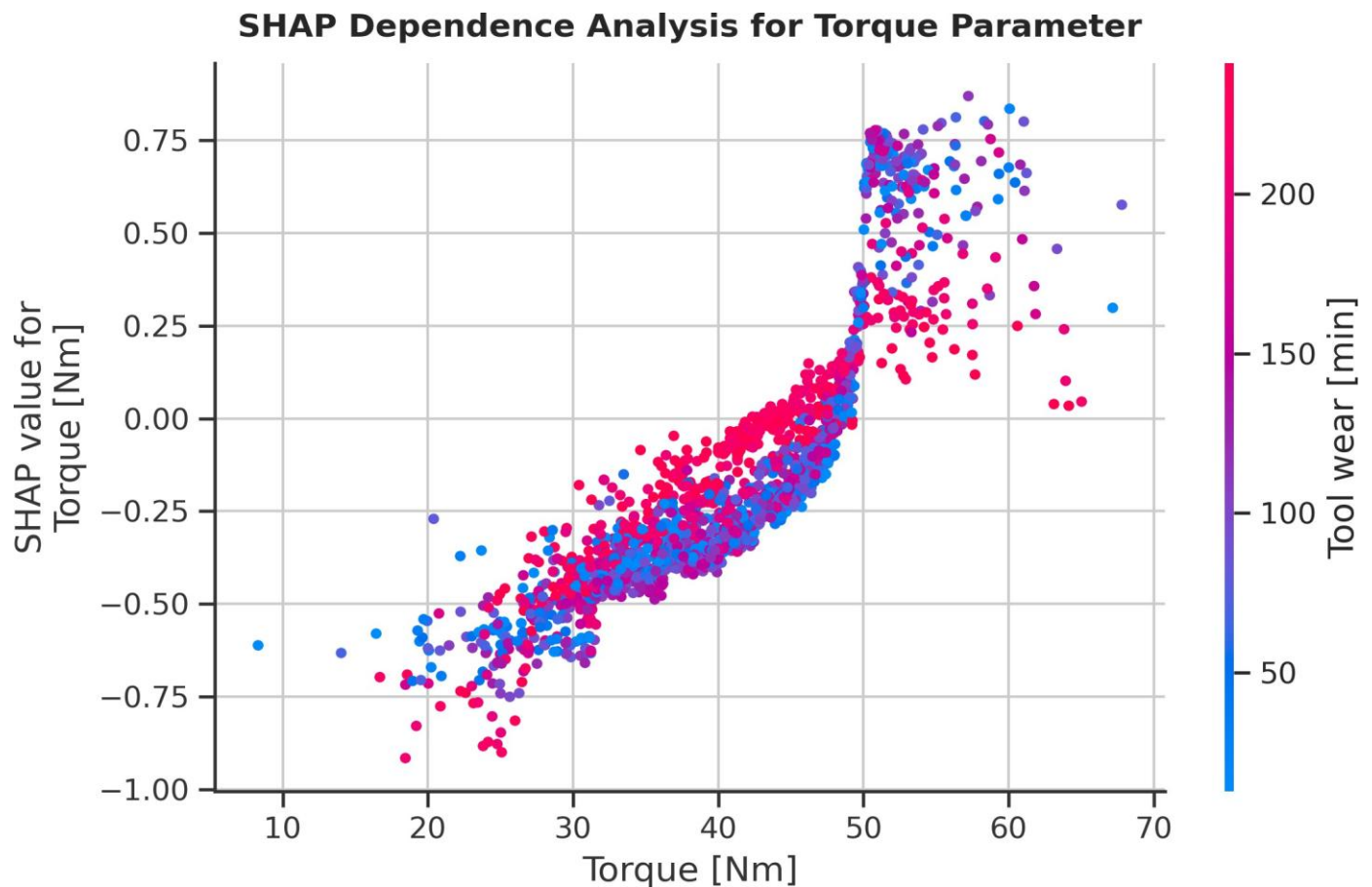
Fig. 10. SHAP dependence plot for torque parameter, revealing nonlinear relationship between torque magnitude and failure prediction contribution. Threshold effect observed near 50 aligns with mechanical design specifications, providing actionable insight for condition-based maintenance thresholds.
