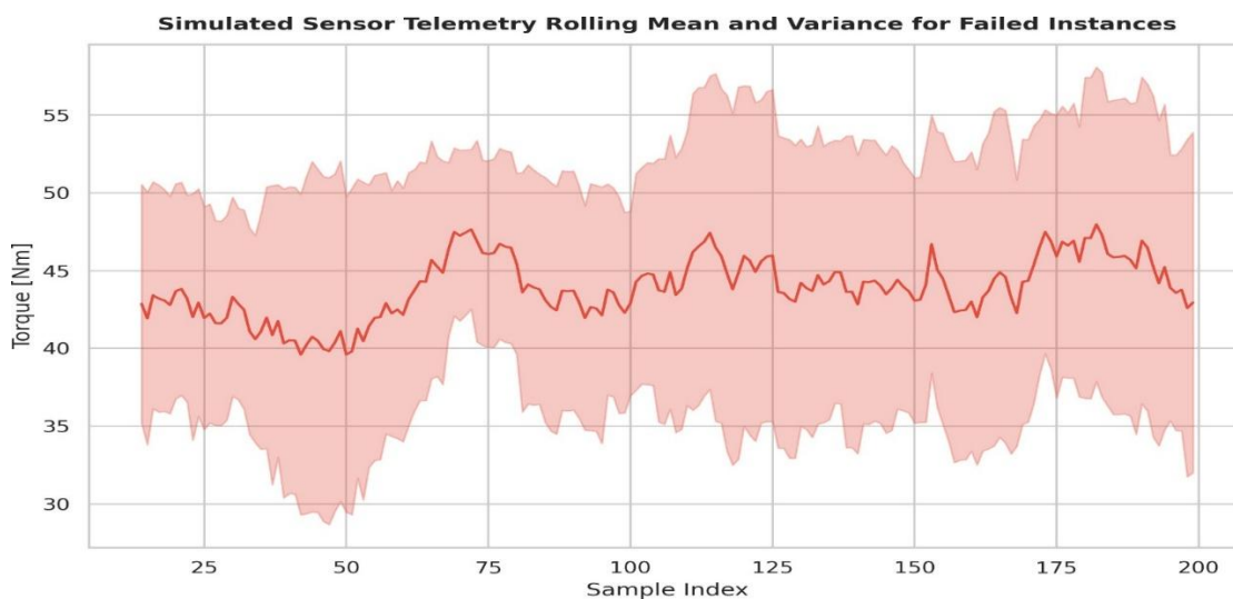
Fig. 14. Simulated sensor telemetry rolling mean and variance for torque parameter in failed instances. Increasing variance preceding failure event enables early anomaly detection via statistical process control methodologies. Rolling window of 15 samples balances responsiveness with noise suppression.
