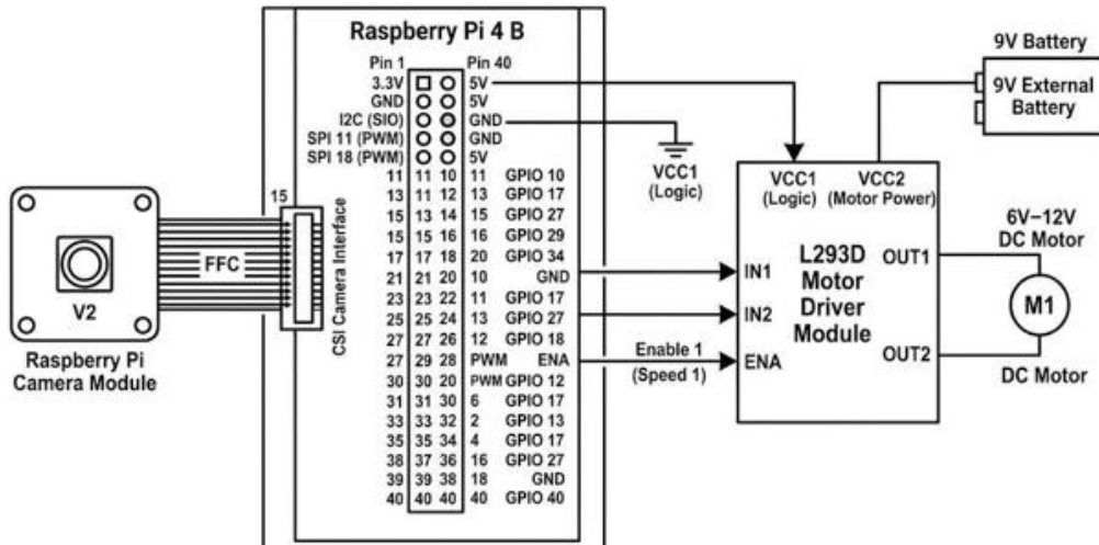
Fig 6.2 Pin diagram of Rover
