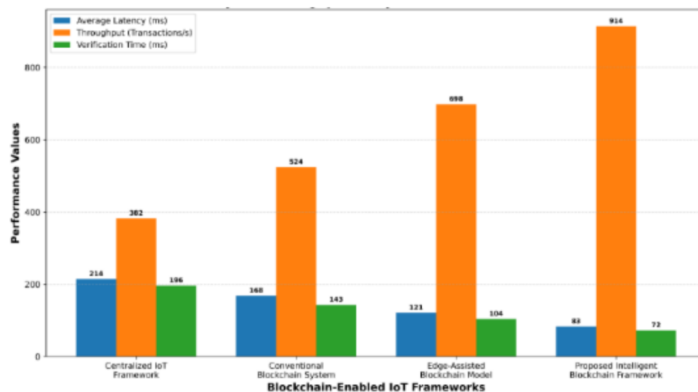
Fig. 3. Comparative Communication Latency and Throughput Analysis of Blockchain-Based IoT Frameworks
