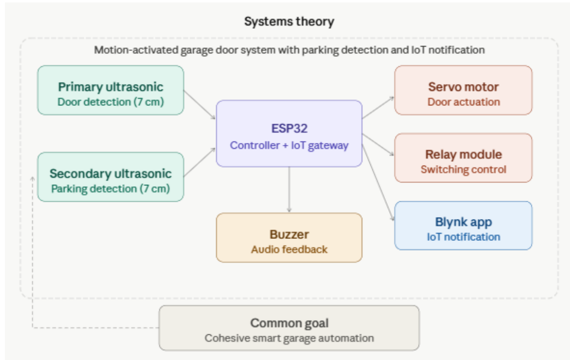
Figure 1. Systems Theory
