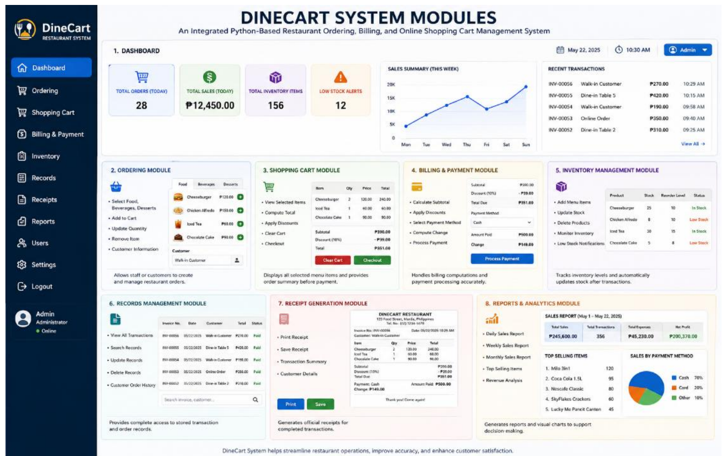
Figure 3. DineCart System Modules Dashboard
