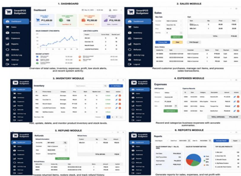
Figure 5. Graphical User Interface of the SmartPOS Budgeteer
