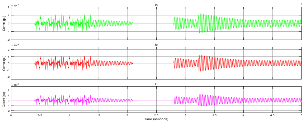
Figure 9: Load current (SVPWM technique)
