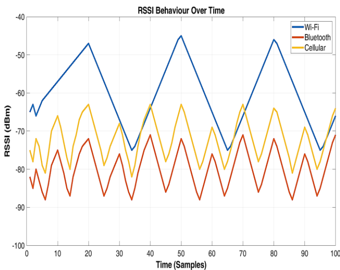
Figure 8a: Combined RSSI variations Output variations
