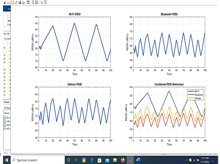
Figure 8b: Wi-Fi, Bluetooth, and Cellular RSSI
