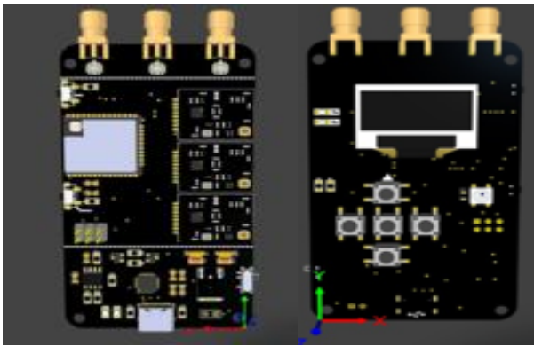
Figure 5: System PCB
