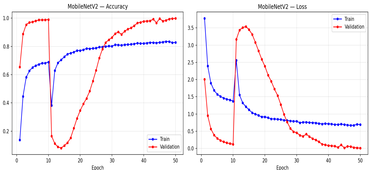
Figure 5. MobileNetV2 training and validation accuracy and loss curve for 50 epochs
