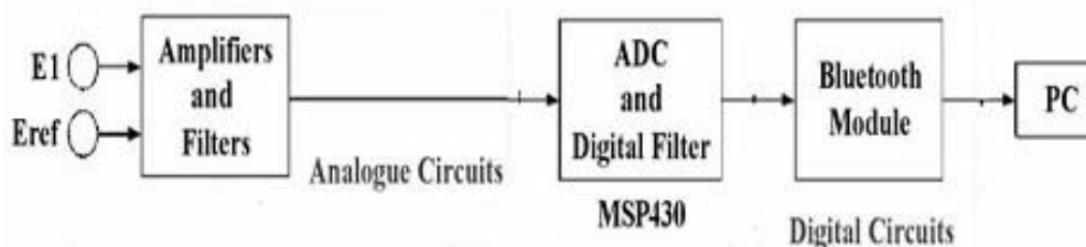
Fig.1. Figure shows the extraction and Wireless transmission of EEG
