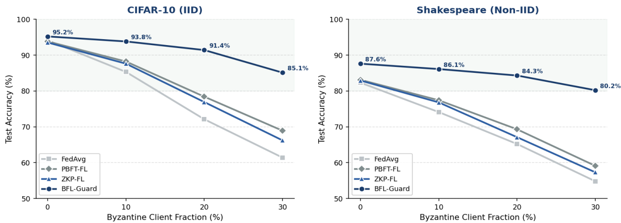
Figure 2. Test accuracy vs. Byzantine client fraction. BFL-Guard maintains robust accuracy where FedAvg and other baselines collapse under adversarial conditions.
