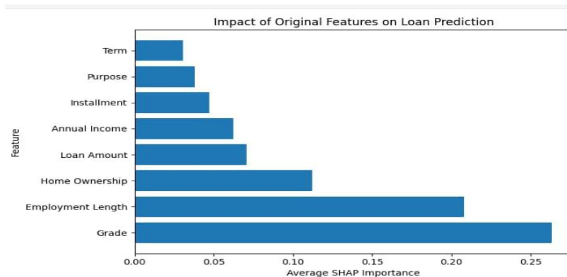
Figure 3: SHAP summary plot for Loan decision model
