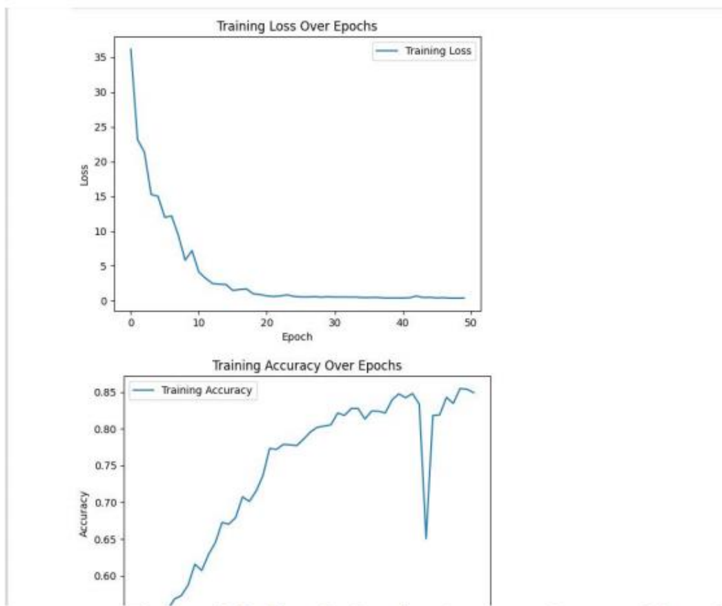
Figure 4: Accuracy and loss rates across training epochs
