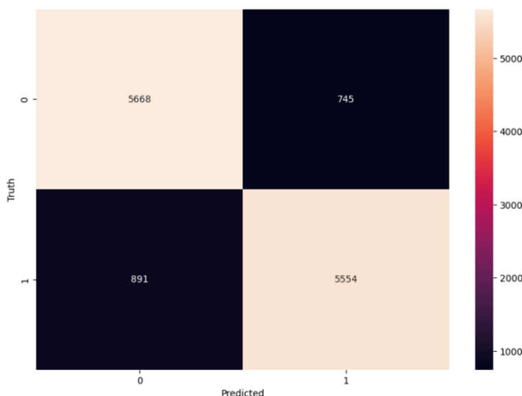
Figure 5: Confusion matrix
