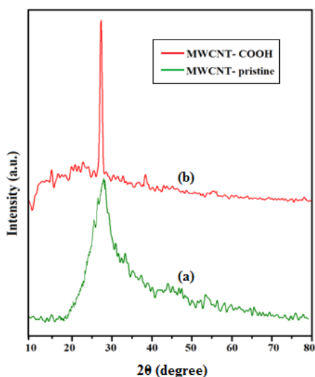
Fig 5.4 XRD patterns of (a) MWCNT-pristine and (b) MWCNT-COOH.
