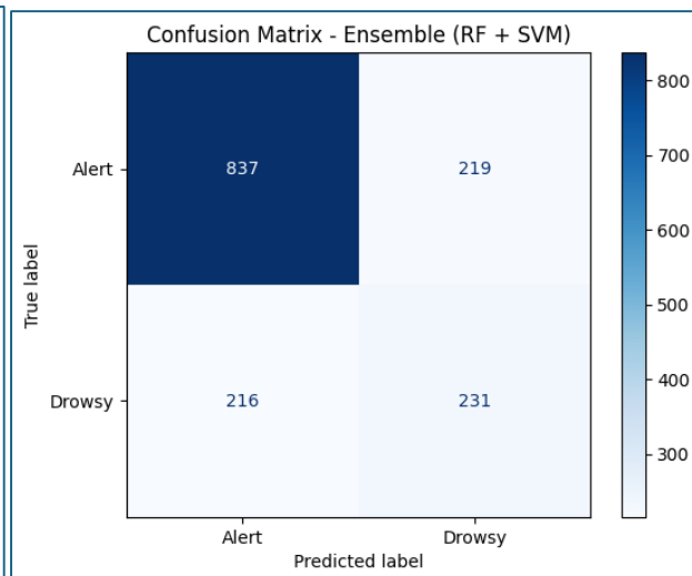
Figure 14: RF+SVM Training Confusion
