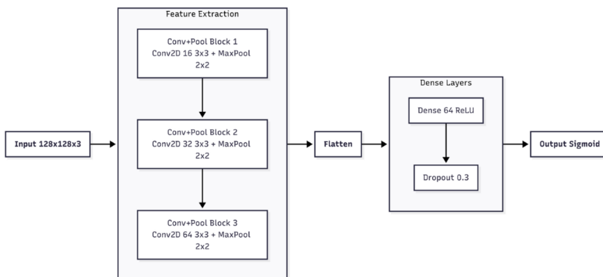
Figure 7: TinyCNN Model Architecture
